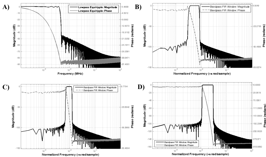
Figure 3.5: The magnitude and phase of each FIR filter: A) delta (0-4 Hz); B) theta (4-8 Hz); C) alpha (8-12 Hz); D) beta (12-30 Hz).
