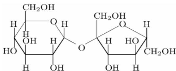
FIG. 2.4 Sacarose - C_{12}H_{22}O_{11}
