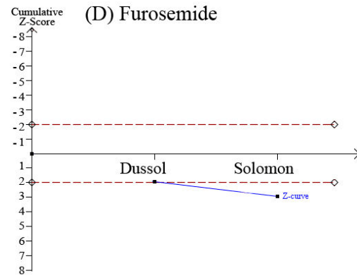
Figure 3. TSA for others pharmacological interventions. The cumulative Z-curves (blue) were constructed with each cumulative Z-value calculated after including a new trial according to publication date. Crossing of the two-sided Z=1.96 (purple) provides a traditionally significant result. Crossing of the trial sequential monitoring boundaries (red) is needed to obtain reliable evidence.
