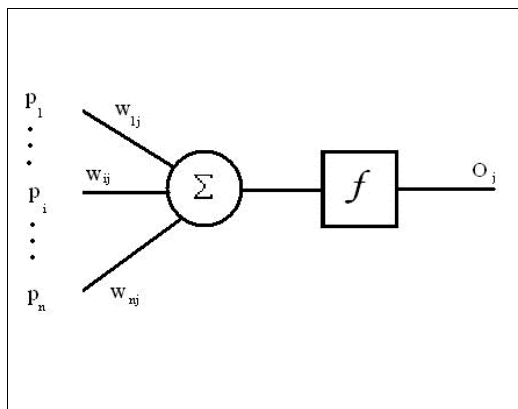
Fig. 2. Artificial Neuron
