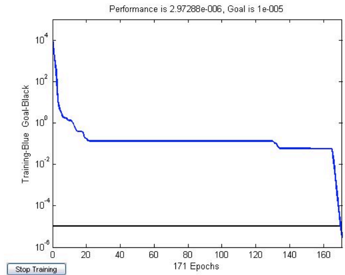
Fig. 6. Network performance
