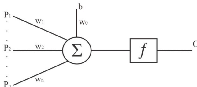
Figura 2.8 – Perceptron
