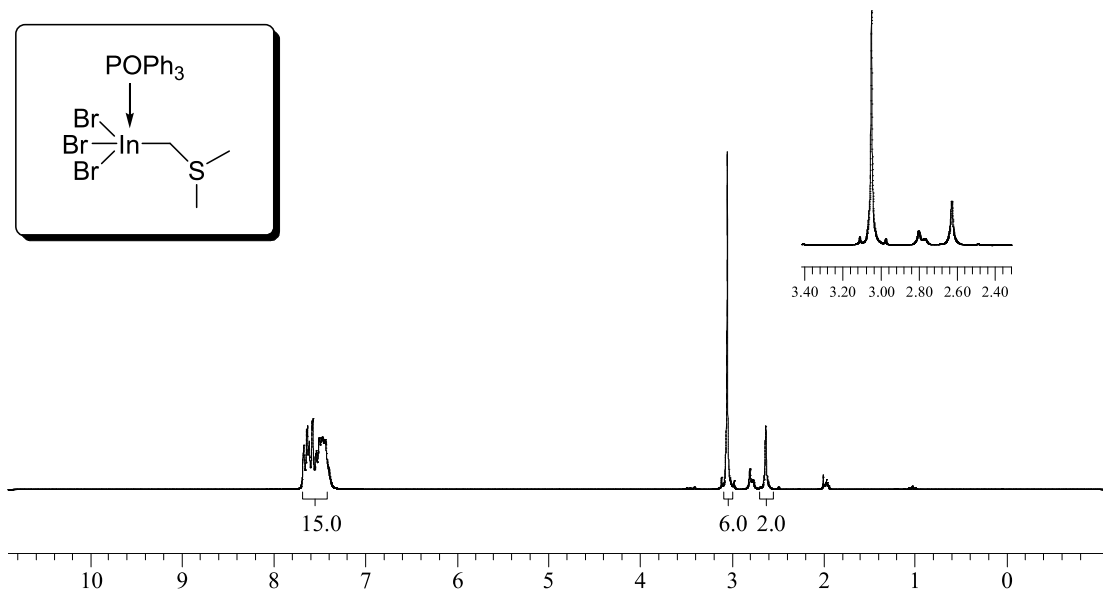
Figura 24. Espectro de RMN de ^1\text{H} em \text{acetona-}d_6 do composto \text{Br}_3\text{In}(\text{Ph}_3\text{PO})\text{CH}_2\text{S}(\text{CH}_3)_2 , 5.
