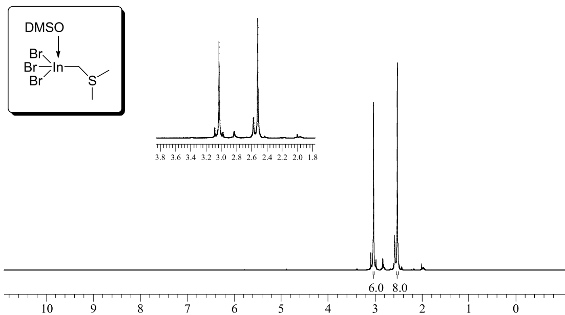
Figura 23. Espectro de RMN de ^1\text{H} em \text{acetona-}d_6 do composto \text{Br}_3\text{In}(\text{DMSO})\text{CH}_2\text{S}(\text{CH}_3)_2 , 4.
