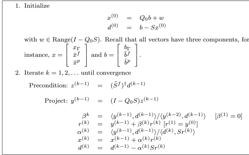
Figure 6.1: Implementation of the projected preconditioned conjugate gradient algorithm for the system (6.14) involving the BDD preconditioner (6.27).
