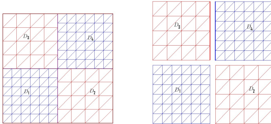
Figure 3.1: On the left picture we display a shape regular triangulation in each subdomain. On the right picture we show finite element meshes in each subdomain.
