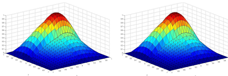
Figure 3.3: Computed (left) and exact solution (3.2) (right) for k_1 = 2 , k_2 = 5 , u_1(x_1) = \sin\left(\frac{\pi*(x+1)}{k_1+1}\right) and u_2(x_2) = 4(x+1)(k_2-x)/(k_2+1)^2 .
