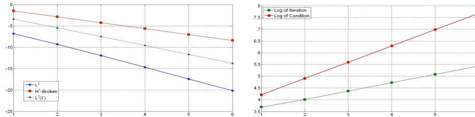
Figure 3.4: Logarithm of the L^2(D) , H^1 -broken, and L^2(\Gamma) errors (left). Logarithm of the iteration and condition number (right).
