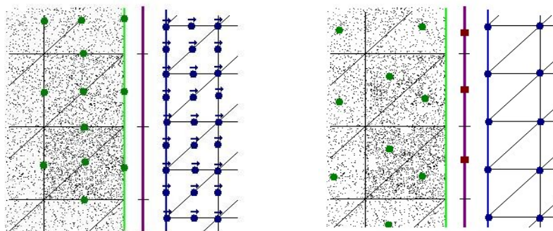
Figure 2.3: On the left picture: degrees of freedom for Raviart-Thomas velocity (left subdomain \bullet ) and Taylor-Hood velocity (right subdomain \vec{\bullet} ). On the right picture: degrees of freedom for Raviart-Thomas pressure (left subdomain \bullet ), Taylor-Hood pressure (right subdomain \bullet ), P_0 elements on the interface for Lagrange multipliers ( \blacksquare ).
