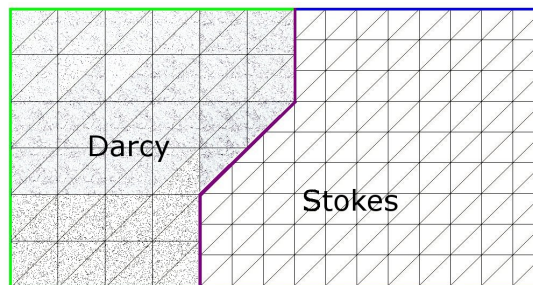
Figure 2.2: Nonmatching triangulations for Darcy-Stokes coupling.
