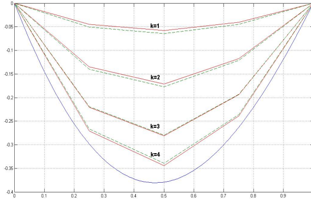
Figure 9.2: Approximation of the coefficient u_{(1,0,0,\dots)} for K = N = k , h = \frac{1}{4} and \epsilon = \frac{1}{2} (solid line) and \epsilon = 0 (dashed line).
