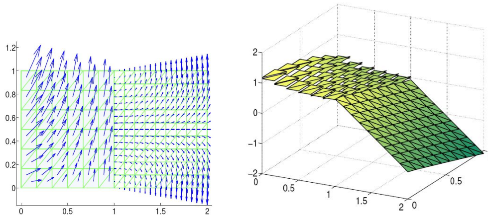
Figure 5.1: Computed velocities (left) and pressures (right). On the porous side we have plot the value of the velocity at the centroid of each triangle.
