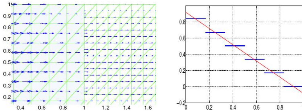
Figure 5.2: The x-component of the discrete velocity (left figure), where on the porous side (left subdomain) we plot the two values of the x component of the velocities at the midpoint of each edge; recall that Raviart-Thomas elements allow discontinuous tangential velocities on interior edges. The discrete (in blue) and the exact (in red) Lagrange multipliers on the interface (right figure).
