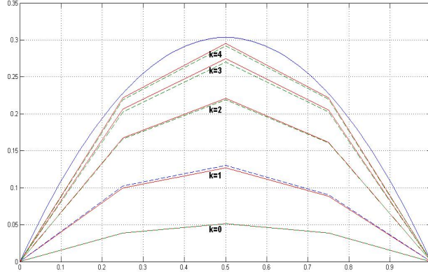
Figure 9.1: Approximation of the coefficient u_{(0,0,0,\dots)} for K = N = k , h = \frac{1}{4} and \epsilon = \frac{1}{2} (solid line) and \epsilon = 0 (dashed line).
