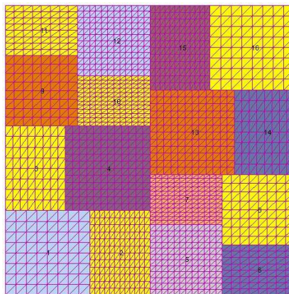
Figure 3.5: Geometrically nonconforming partition of D with a shape regular triangulation in each subdomain.
