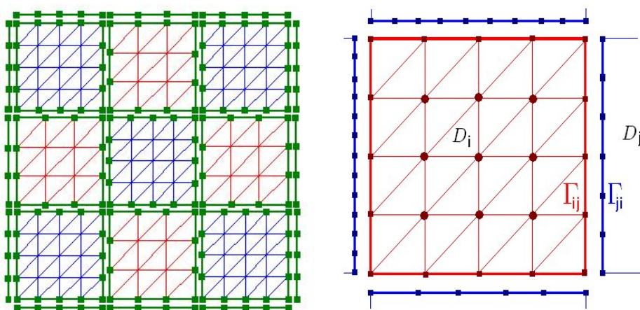
Figure 3.2: On the left: Degrees of freedom associated to \Gamma , the disjoint union of \partial D_i , i = 1, 2, \dots, N , (■). In this case the square subdomain D is the union of 3 \times 3 square subdomains D_i , i = 1, 2, \dots, 9 . On the right: Local degrees of freedom associated to D_i . They are classified in interior (●) and boundary (■) degrees of freedom.
