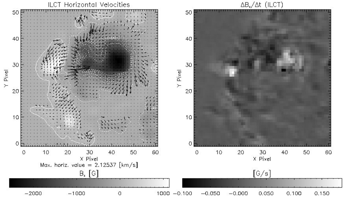
FIGURE 2.8 - Velocity obtained using ILCT method(left) and the variation of the vertical component calculated using \frac{\Delta B_z}{\Delta t} = -\vec{\nabla} \cdot (u^{(ILCT)} B_z) (right). The gray scale represents the intensity or the variation of the LOS component of the magnetic field. The arrows represent the horizontal component of the velocity, with the largest length of the arrow associated to the maximum horizontal value measured for the velocity. The contour lines are drawn for the magnetic field magnitude equal to 300, 500, 700, 900, 1100 and 1300 G.
