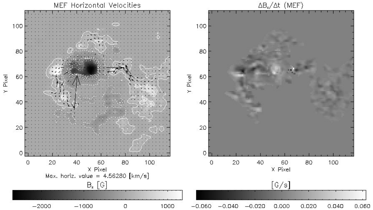
FIGURE 2.4 - Velocity obtained using MEF method (left) and the variation of the vertical component calculated using \frac{\Delta B_z}{\Delta t} = -\vec{\nabla} \cdot (u^{(MEF)} B_z) (right). The gray scale represents the intensity or the variation of the LOS component of the magnetic field. The arrows represent the horizontal component of the velocity, with the largest length of the arrow associated to the maximum horizontal value measured for the velocity. The contour lines are drawn for the magnetic field magnitude equal to 100, 500, 700, 900, 1100 and 1300 G.
