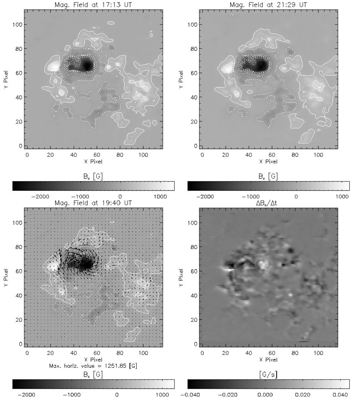
FIGURE 2.1 - Input data used to calculate the velocity fields on May 1 st 1998: a) top left- vertical component of the magnetic field obtained at 17:13 UT, b) top right - vertical component of the magnetic field obtained at 21:29 UT, c) bottom left - vector magnetic field obtained at 19:40 UT and d) bottom right - variation of the vertical component of the magnetic field between 17:13 UT and 21:29 UT. The gray scale represents the intensity or the variation of the LOS component of the magnetic field. The arrows represent the horizontal component of the magnetic field, with the largest length of the arrow associated to the maximum horizontal value measured for the magnetic field. The contour lines are drawn for the magnetic field modulus equal to 100, 500, 700, 900, 1100 and 1300 G.
