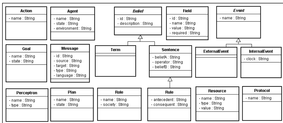
Figura 4.3 – Diagrama de Classes UML do pacote concepts .
