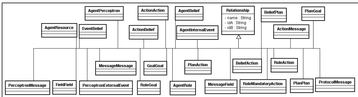
Figura 4.10 – Diagrama de Classes UML do pacote relationships .
