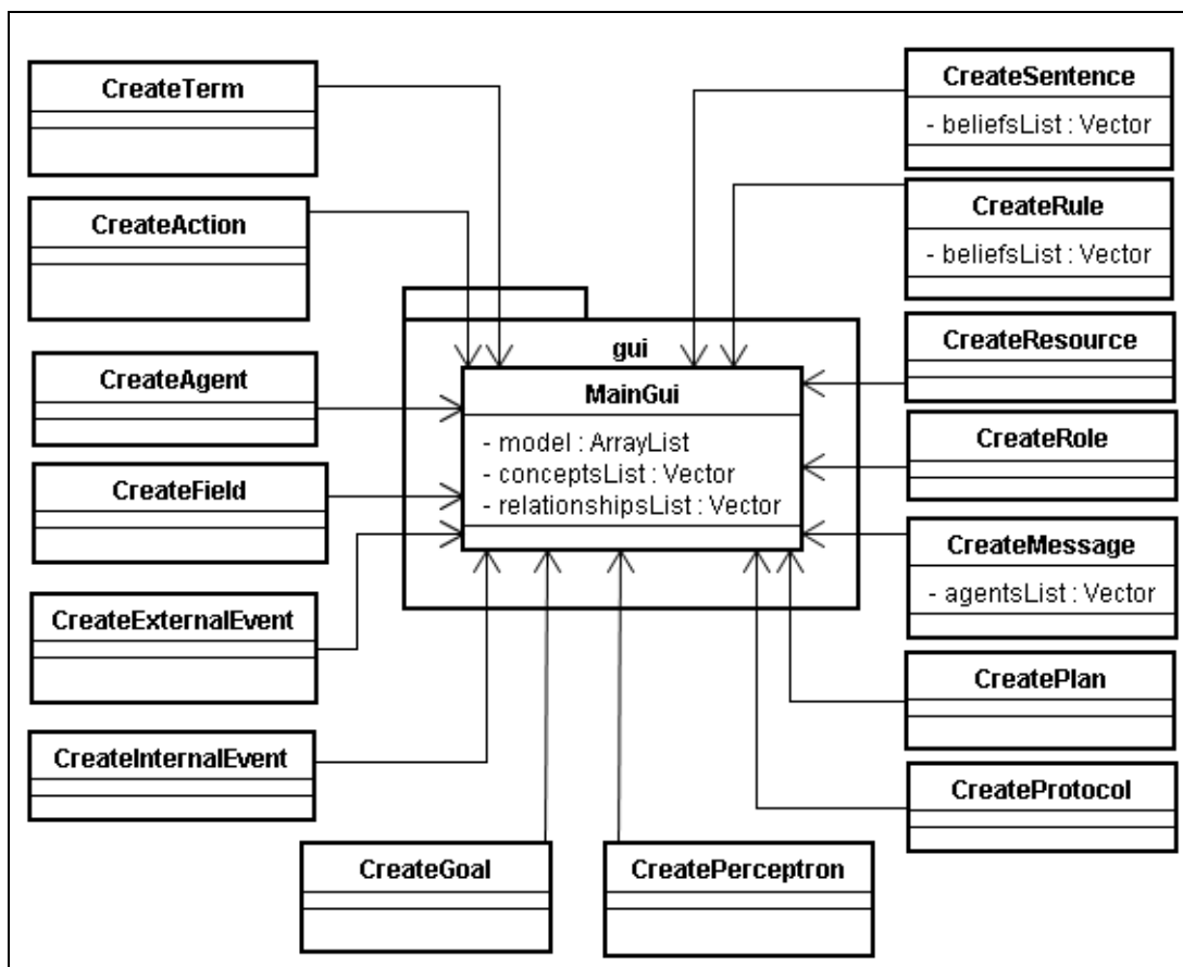
Figura 4.7 – Diagrama de Classes UML do pacote gui.register.concepts .
