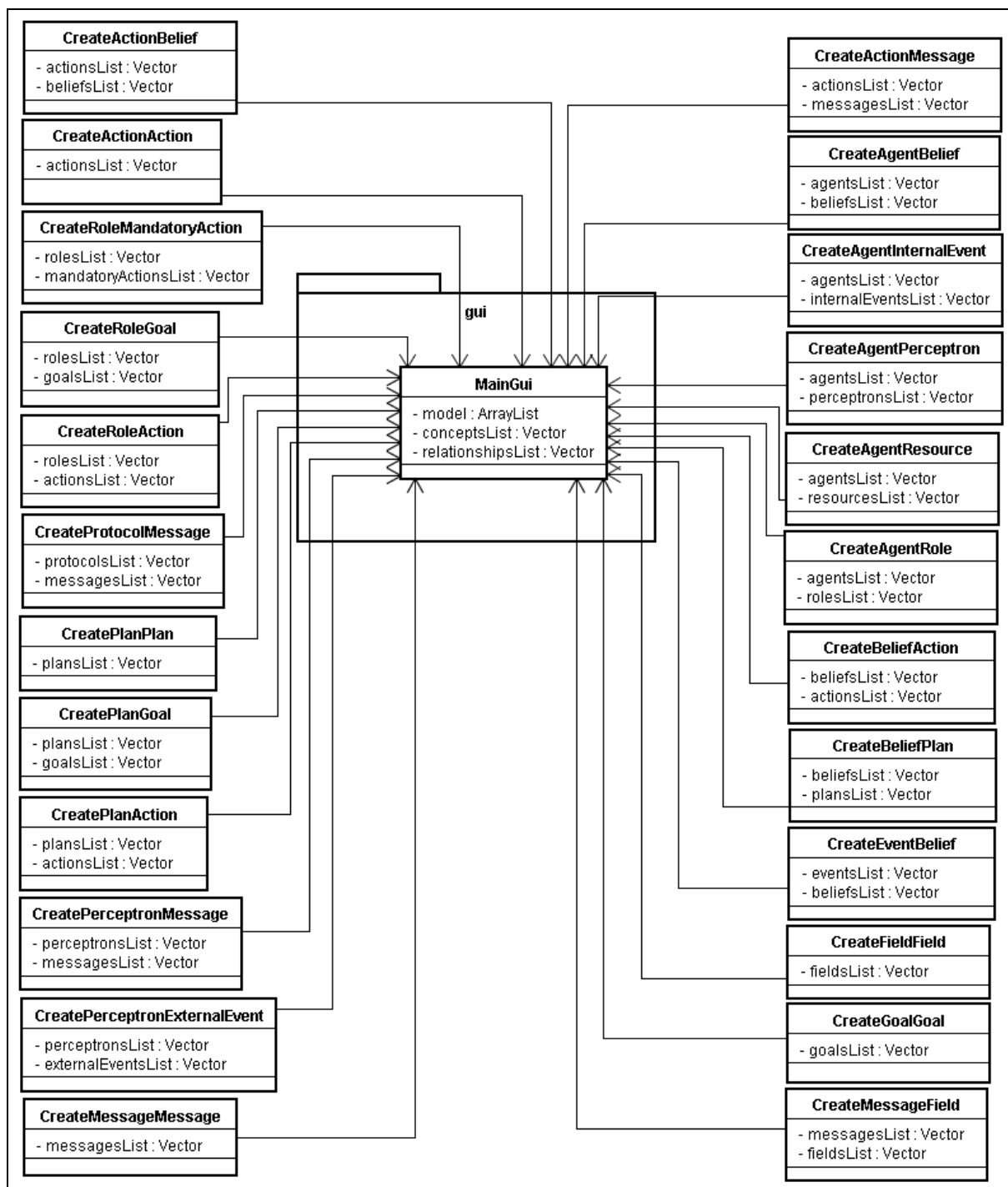
Figura 4.8 – Diagrama de Classes UML do pacote gui.register.relationships .
