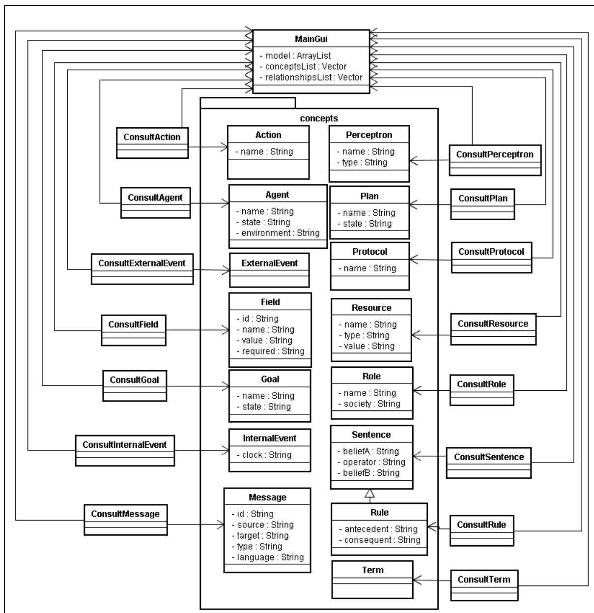
Figura 4.5 – Diagrama de Classes UML do pacote gui.consult .
