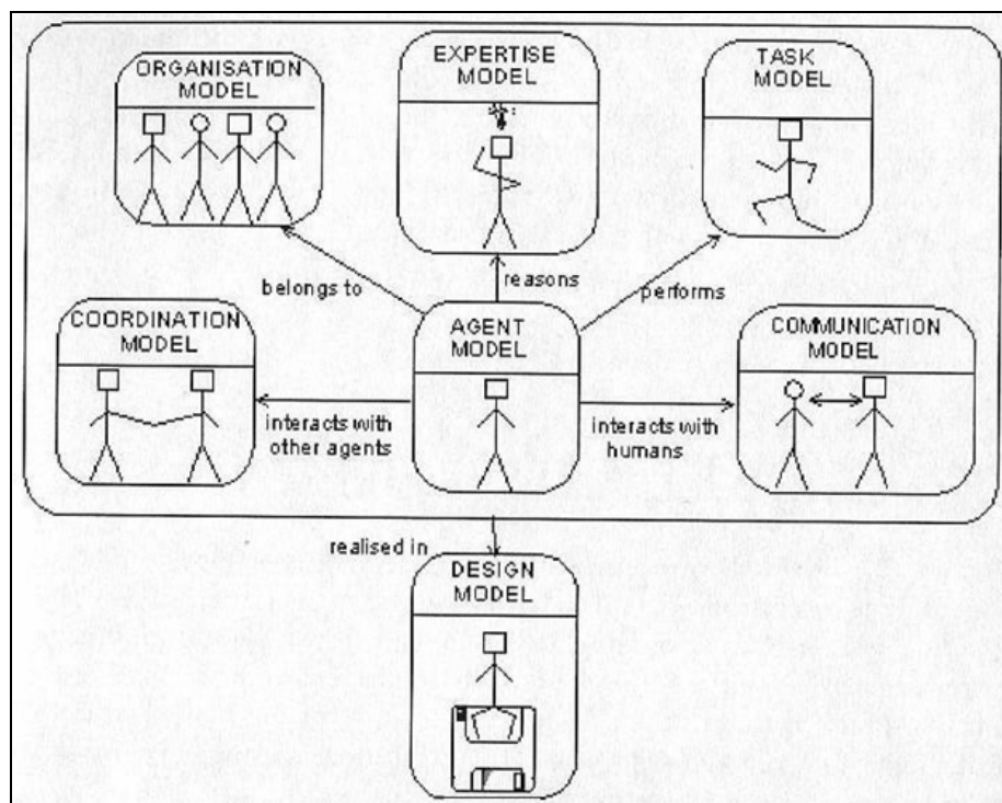
Figura 2.15 – Modelos do MAS-CommonKADS [HEN05].
