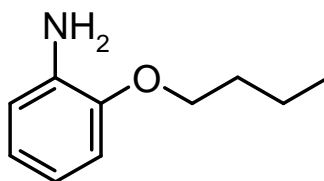
Figura 36 – o -Butoxianilina
