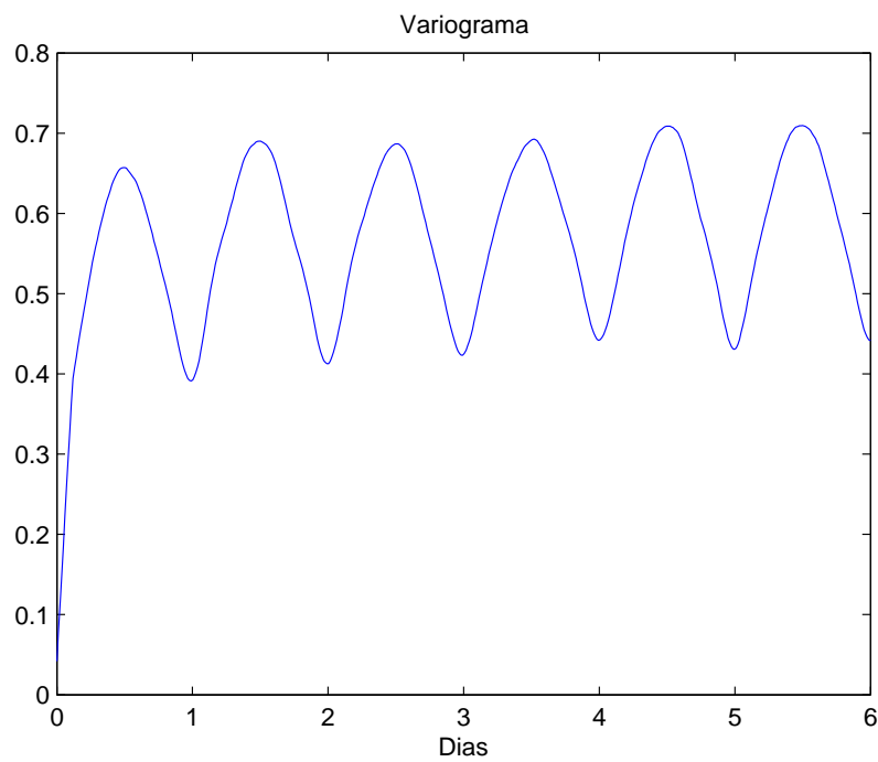
Figura 4.7: Variograma IBOVESPA (2006)
