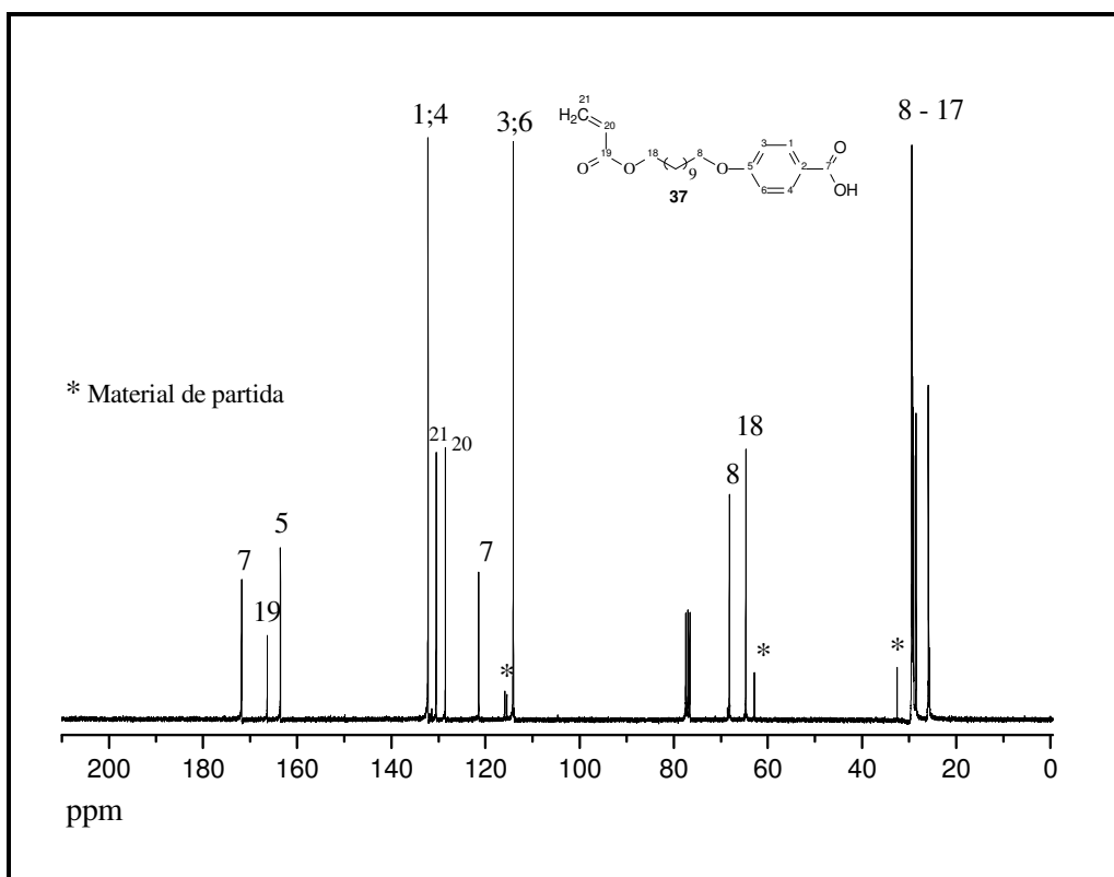
Espectro de RMN ^{13}\text{C} ( \text{CDCl}_3 ), 75 MHz do composto 37
