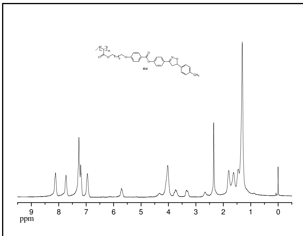
Espectro de RMN ^1\text{H} ( \text{CDCl}_3 ), 300 MHz do composto 41d
