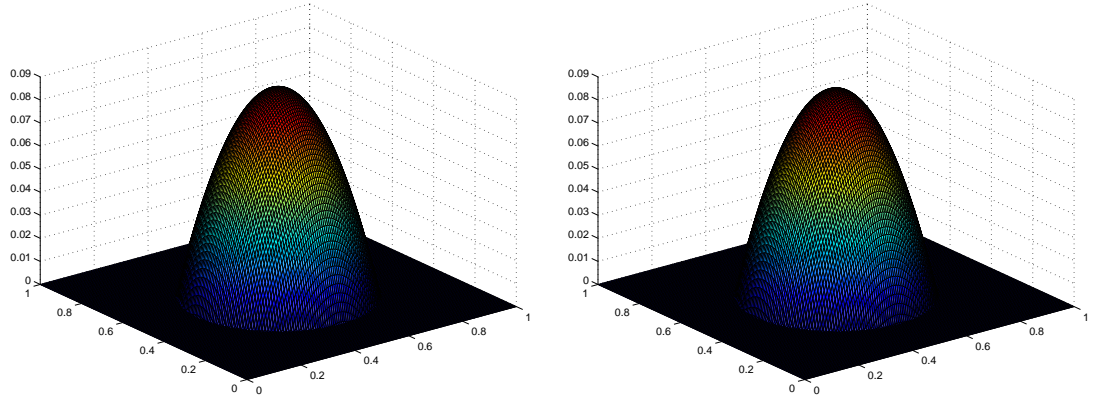
Figure 5.1: Exact solution (left) of problem (5.1) and its B-spline approximation (right) using w\mathcal{B}_h^n(\Omega) .
