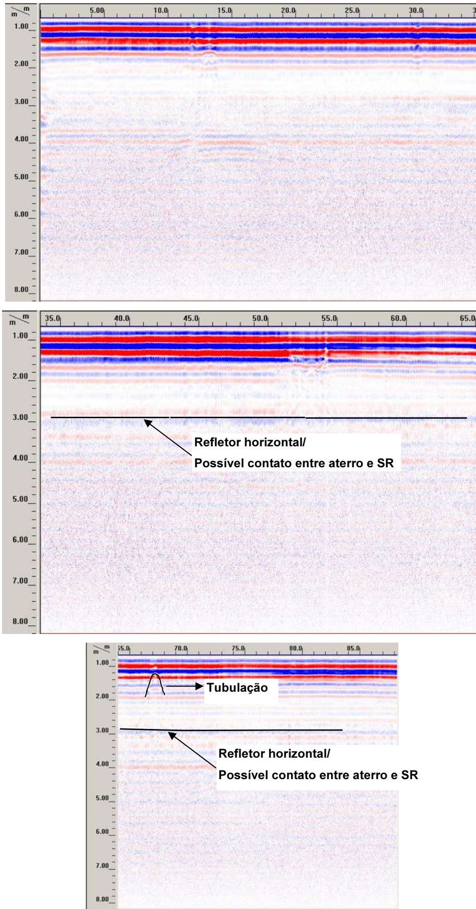
Figura 6.8 – Radargrama no topo do talude
