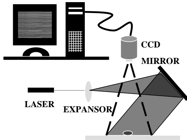
FIGURE 1: Equipment set-up
