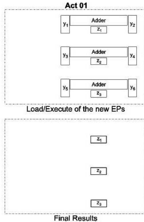
Figure 4: MACs in a DR-FPGA using EPs (accumulating phase)
