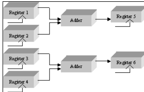
Figure 4: Computation with dynamic reconfiguration - first step
