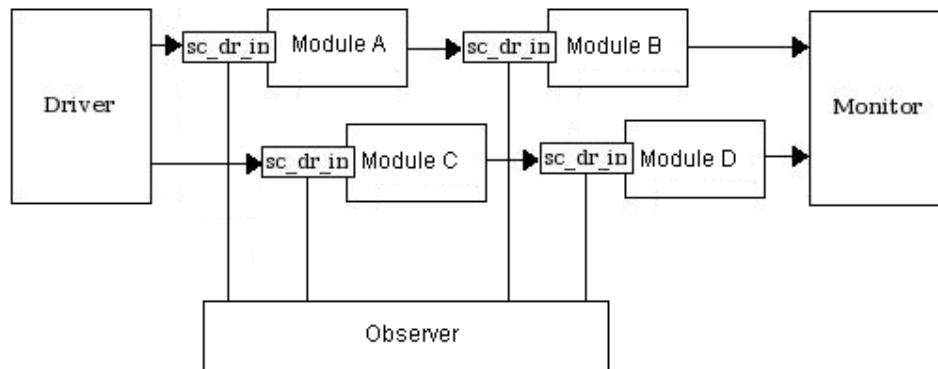
Figure 6: Example showing how sc_dr_in can be connected to modules.
