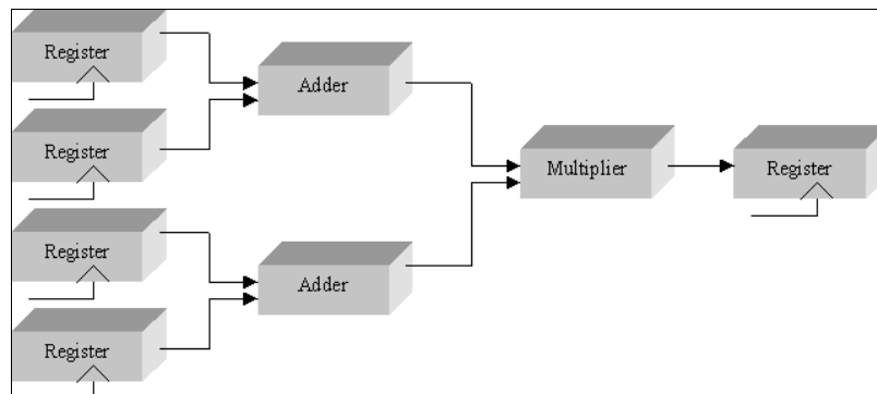
Figure 3: computational model without dynamic reconfiguration
