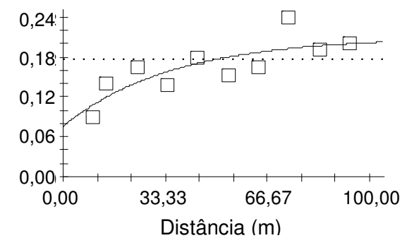
Figura 11. Semivariograma para consumo ponderal ( C_{POND} )
