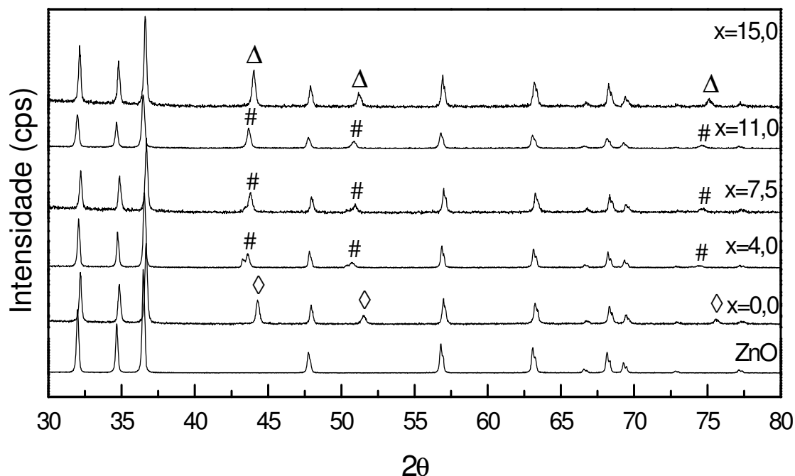
Figura 4.5 – Difratogramas das amostras de \text{Cu}_{15-x}\text{Ni}_x\text{ZnO} , onde x=0, 4, 7,5, 11 e 15 . \text{Cu}^0(\diamond) , \text{Ni}^0(\Delta) e \text{Cu}^0\text{-Ni}^0(\#) .
