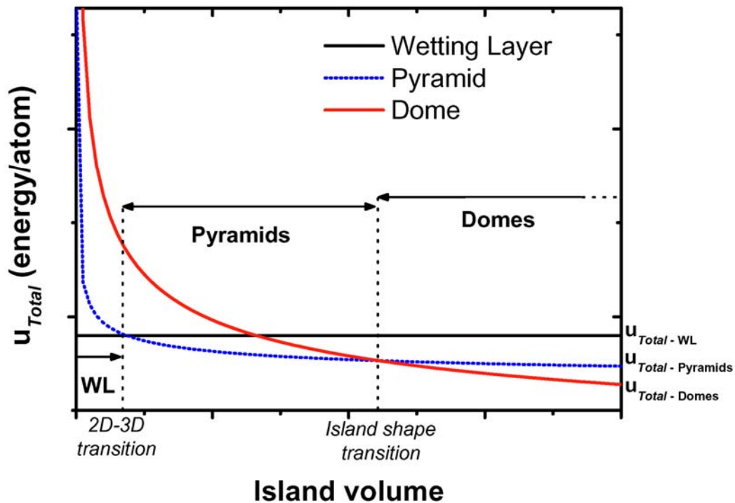
Fig. 2.3 – Phenomenological model for Stranski-Krastanov island shape transition [Shchukin95]. The WL per-atom total energy is constant (horizontal solid line). Dashed vertical lines indicate regions where the growth of WL, pyramids (dashed curve) or domes (solid curve) is favored over the other structures.
