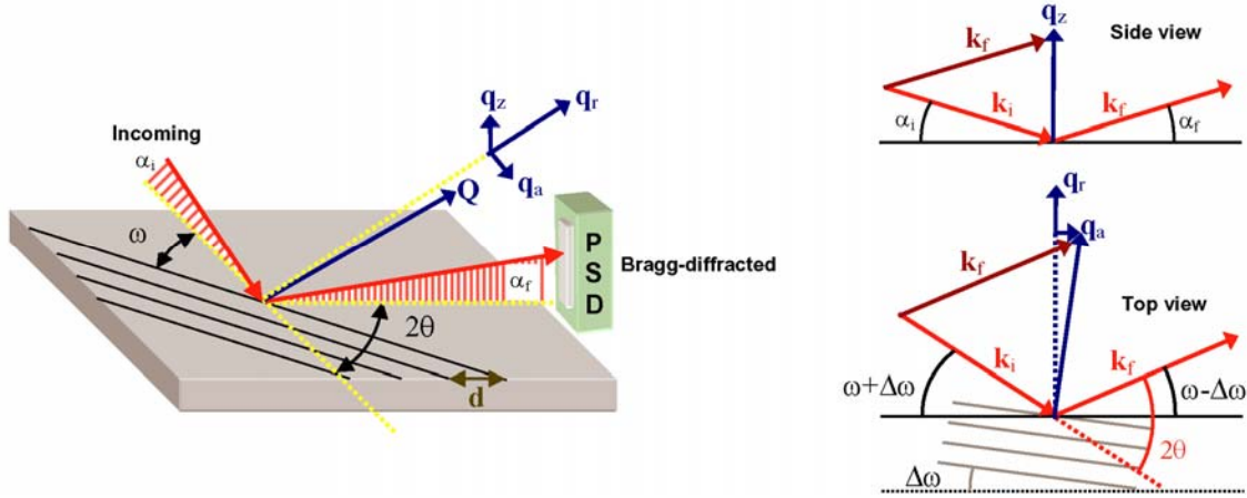
Fig. 1.11 – Grazing-Incidence Diffraction geometry. The x-ray beams are represented in red while the momentum transfer vectors were drawn in blue. The radial ( \mathbf{q}_r ), angular ( \mathbf{q}_a ) and vertical ( \mathbf{q}_z ) components of momentum transfer are shown in detail on the right.
