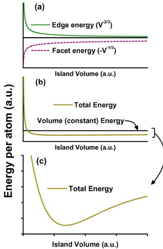
Fig. 3.11 – (a) Sketch of the edge and facet energy terms (per atom) of eq. 3.4 as a function of the island volume. (b) Variation of the total energy per atom ( u_{Total} – eq. 3.4) with the island volume. (c) Expanded energy scale (zoom) of u_{Total} shown in (b); the minimum position defines the equilibrium size of the islands.
