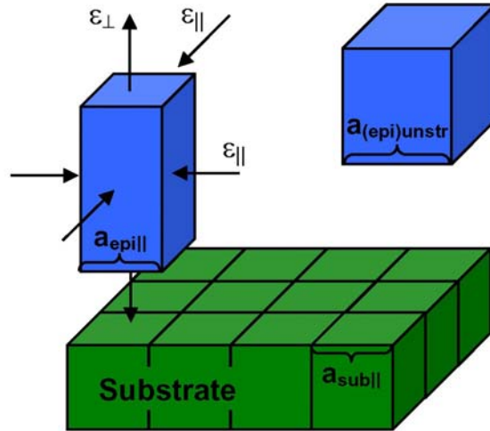
Fig. 2.1 – Sketch of the strains and lattice parameters for heteroepitaxial deposition under biaxial strain. The film unit cells develop strains \epsilon_{\perp} and \epsilon_{\parallel} related by eq. 2.11
