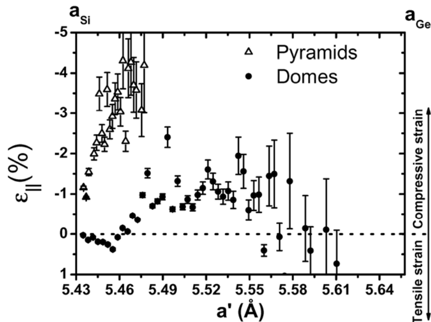
Fig. 2.12 – In-plane strain \epsilon_{\parallel} as a function of a' for pyramids and domes. The x-axis of this graph spans from Si to Ge bulk lattice parameter value. The horizontal dashed line corresponds to zero strain condition; i.e., that of a SiGe unstressed alloy. Regions below and above the dashed line correspond to tensile and compressive strain, respectively.
