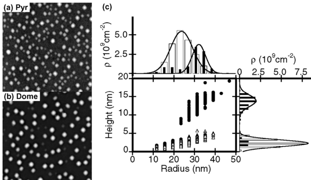
Fig. 2.4 – 1µm 2 AFM images of Pyramid (a) and Dome (b) samples. Note the smaller size of the pyramid islands. The shape of these islands is not completely clear from the measurements due to tip convolution effects. (c) Statistical analysis performed in a 4µm 2 area; open symbols and bars correspond to the pyramid sample whereas solid ones correspond to the dome sample. It can be seen quite clearly the different island types from the height x radius plot.
