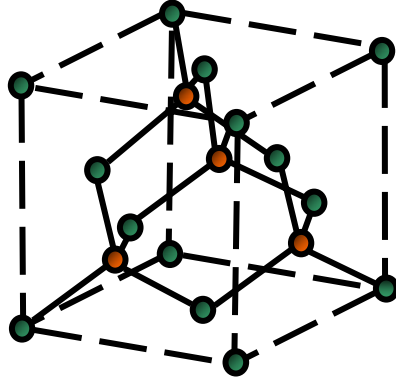
Fig. 1.8 – SiGe zincblend (pseudodiamond) unit cell. Si atoms are represented in green while Ge atoms appear in orange.
