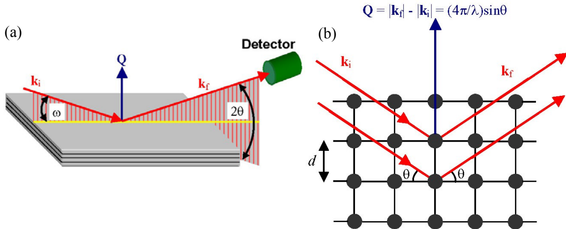
Fig. 1.9 – (a) Geometry used for coplanar x-ray diffraction. (b) Sketch of Bragg's law in reciprocal space. The usual formula n\lambda = 2d\sin\theta can be obtained assuming |\mathbf{Q}| = n2\pi/d .
