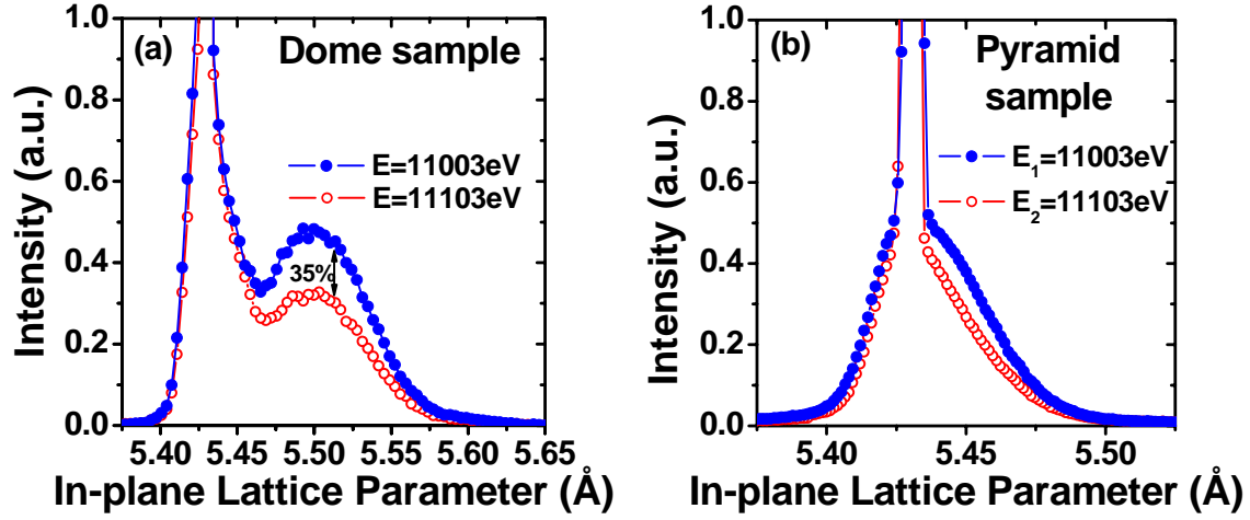
Fig. 2.10 – X-ray radial scans along the (220) direction using two different x-ray photon energies near the Ge K-edge for the dome (a) and pyramid (b) samples. The q_r axis was directly converted to in-plane lattice parameter. The arrow indicates where the difference of intensity is \sim 35\% , i.e. where the island is pure Ge.
