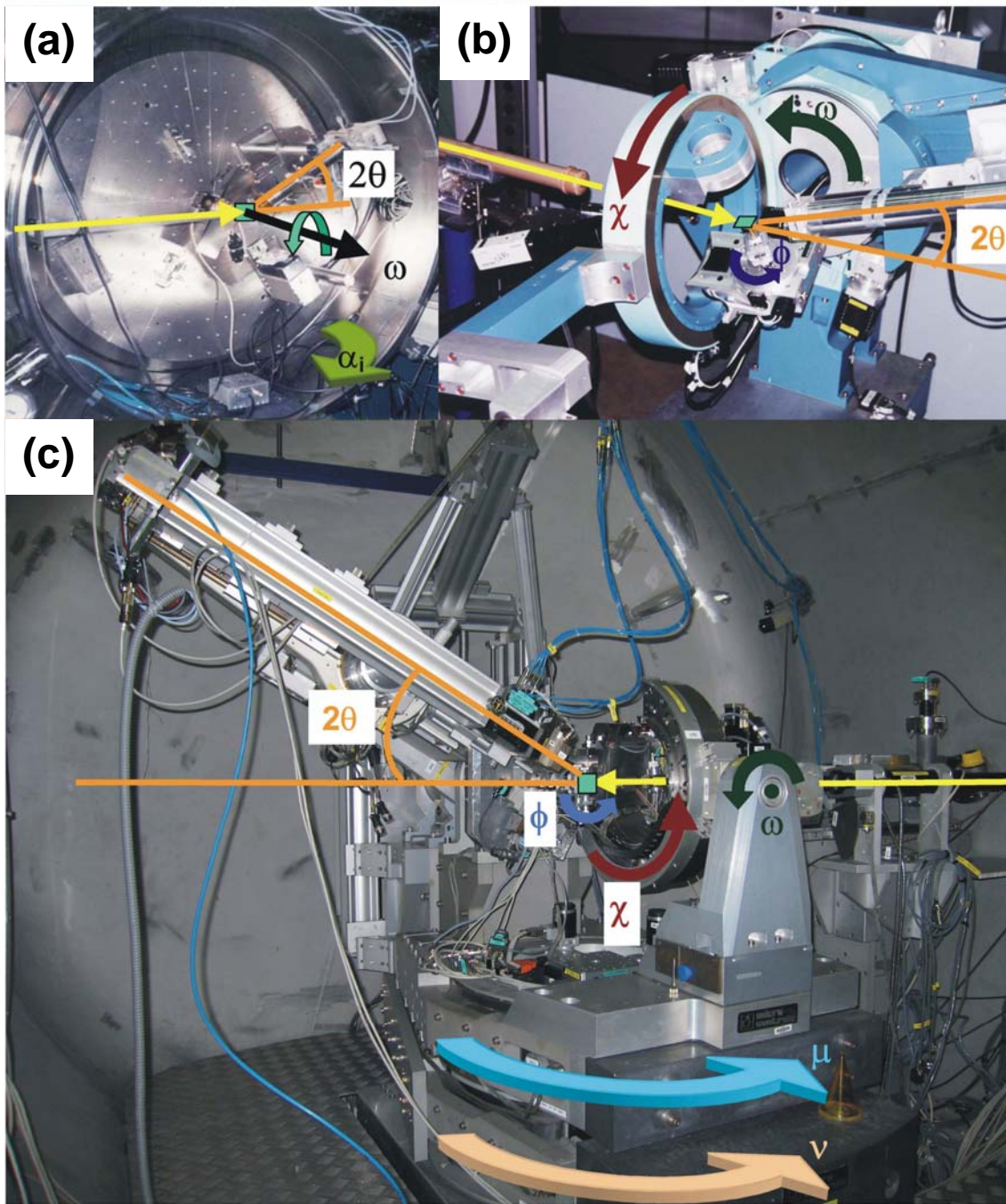
Fig. 1.3 – Diffractometers of (a) XDR1 and (b) XRD2 beamlines at LNL and (c) ID01 beamline at ESRF. The x-ray path is indicated by the yellow line while diffractometer movements are represented by arrows.
