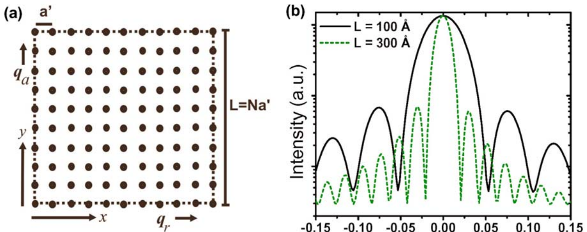
Fig. 2.7 – (a) Sketch of a square section inside an island. (b) Angular profiles generated by eq. 2.15 for L = 100 \text{ \AA} (solid line) and L = 300 \text{ \AA} (dashed line).
