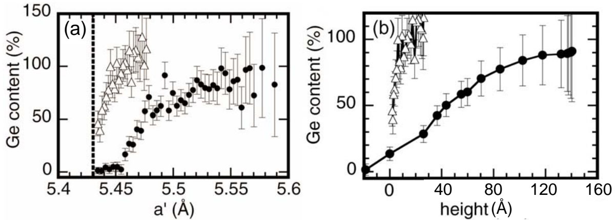
Fig. 2.11 – (a) Ge concentration as a function of local lattice parameter (obtained using eq. 2.15) for both pyramids (triangles) and domes (circles). (b) Ge content as a function of height obtained from a comparison of x-ray anomalous scattering results and typical atomic force microscopy images for both pyramids (triangles) and domes (circles). Mudar fig.b para Ge content.
