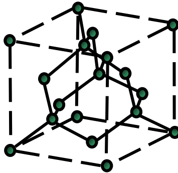
Fig. 1.7 – Diamond (Si or Ge) unit cell.
