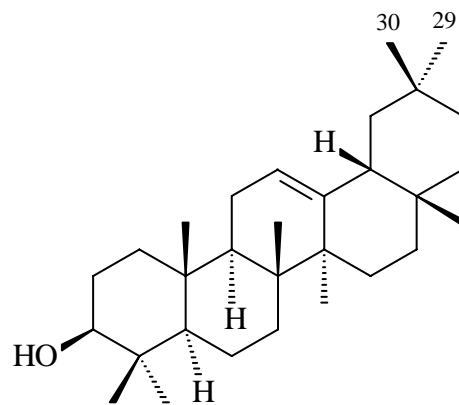
\beta - amirina
