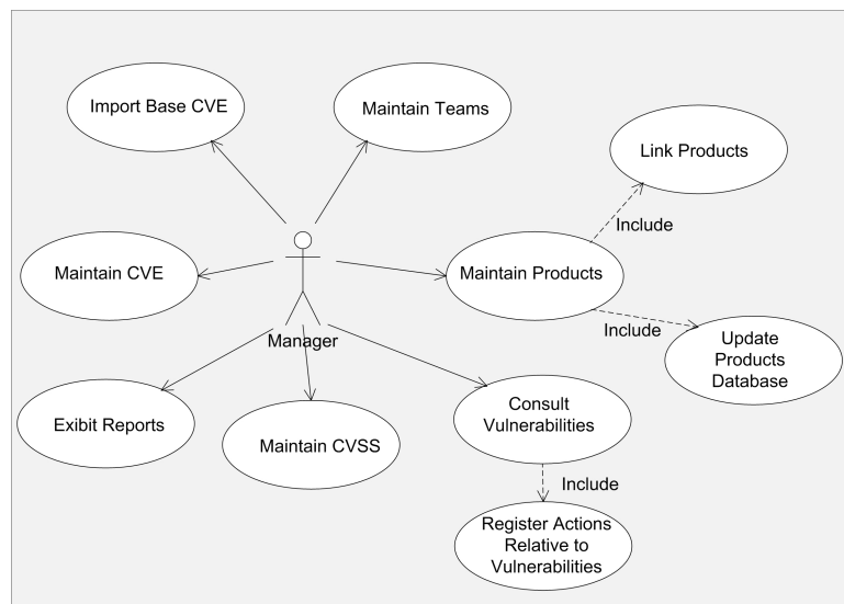
Figure 9.3: Diagram of the Manager's perspective
