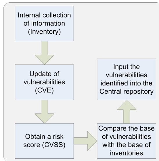
Figura 9.6: Procedures for Risk Analysis in the context of the proposed framework
