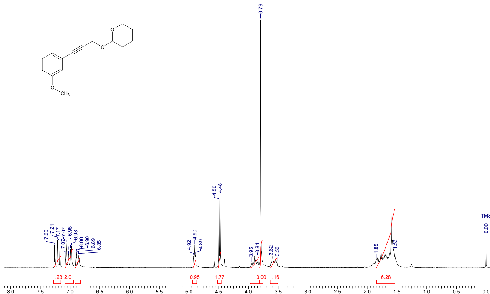
Espectro de RMN 1 H do 2-([3-(3-metoxifenil)prop-2-in-1-il]oxi}tetraidro-2H-pirano (41a)
