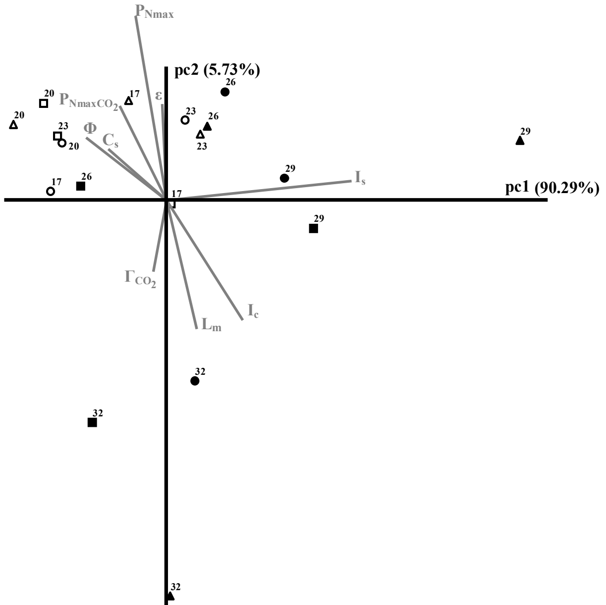
Figure 8. Principal component analyses of leaf gas exchange obtained under elevated (solid symbols) and reduced (open symbols) temperatures in three Coffea arabica cultivars (Catuaí Vermelho □, ■; Obatã, ○, ●; and Ouro Verde Δ, ▲). Temperatures are indicated above each symbol. Vectors (grey lines) represent main physiological variables influencing symbols distribution. P_{Nmax} = maximum net photosynthesis, P_{NmaxCO_2} = photosynthetic capacity, \epsilon = apparent carboxylation efficiency, L_m = mesophyll limitation of net photosynthesis, \Phi = apparent quantum efficiency, I_s = light saturation point, I_c = light compensation point, C_s = CO_2 saturation point, and \Gamma_{CO_2} = CO_2 compensation point.
