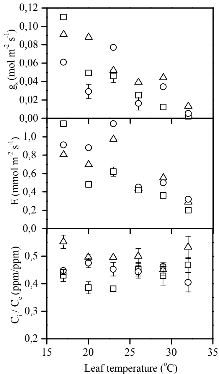
Figure 5. Stomatal conductance ( g_s ), leaf transpiration ( E ) and intercellular ( C_i ) per external ( C_e ) \text{CO}_2 concentration in leaves of Coffea arabica , cultivars Catuai Vermelho \square , Obatã \circ , and Ouro Verde \triangle under photosynthetic photon flux density higher than 1200 \mu\text{mol m}^{-2} \text{s}^{-1} and regular atmospheric \text{CO}_2 concentration ( 355 \mu\text{mol mol}^{-1} ) as a function of leaf temperature. Each symbol represents mean ( 32 < n < 43 ) and bars the standard error.
