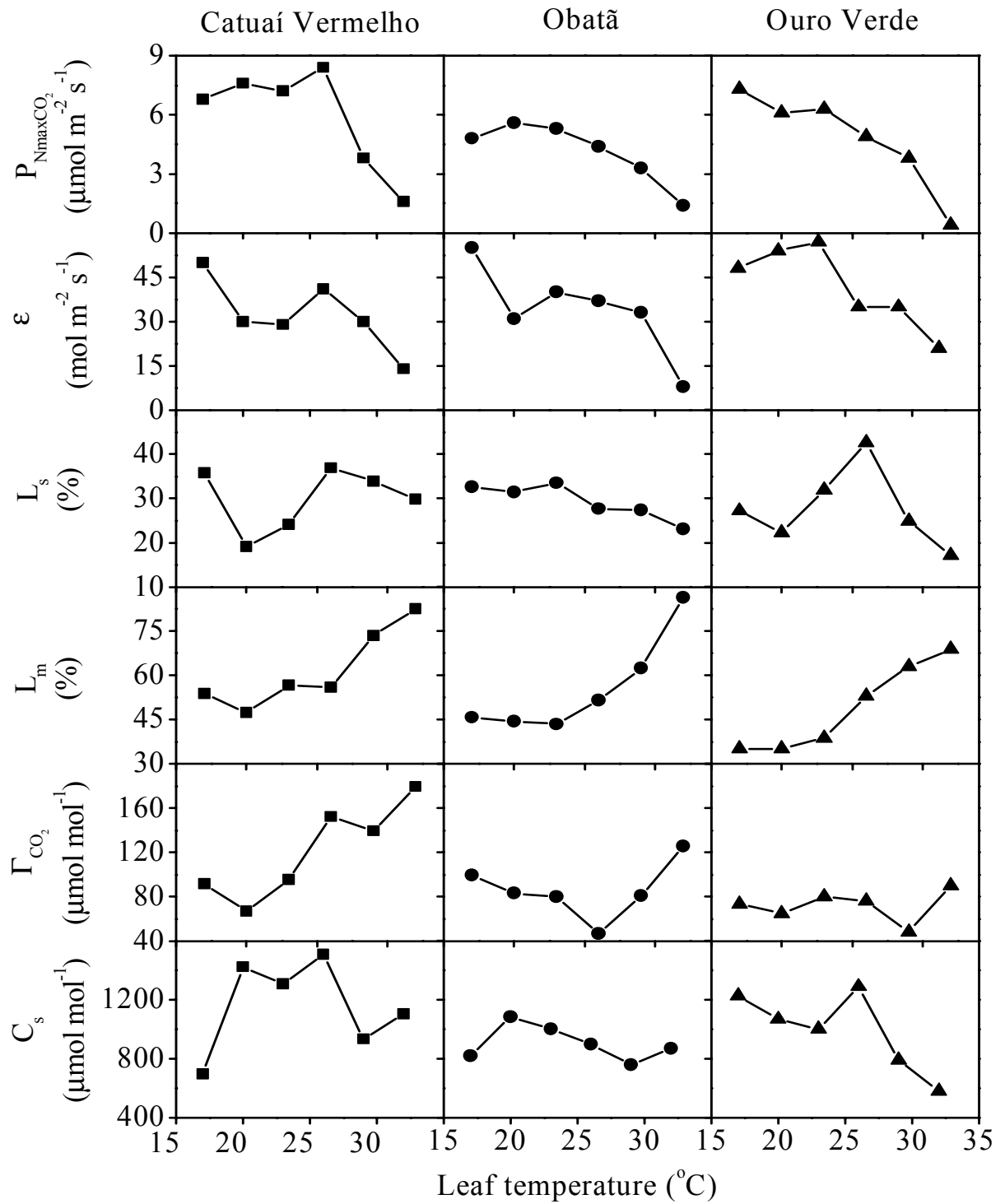
Figure 7. Photosynthetic capacity ( P_{N_{maxCO_2}} , \mu\text{mol m}^{-2} \text{s}^{-1} ), apparent carboxylation efficiency ( \epsilon , \text{mol m}^{-2} \text{s}^{-1} ), stomatal ( L_s , %) and mesophyll ( L_m , %) limitations of photosynthesis, \text{CO}_2 compensation point ( \Gamma_{\text{CO}_2} , \mu\text{mol mol}^{-1} ), and \text{CO}_2 saturation point ( C_s , \mu\text{mol mol}^{-1} ) on leaves of Coffea arabica , cultivars Catuaí Vermelho (■), Obatã (●), and Ouro Verde (▲) after 14 hours under 17, 20, 23, 26, 29, and 32°C.
