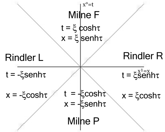
FIG. 1: The Minkowski spacetime divided into four coordinate systems (trivial coordinates are omitted)
