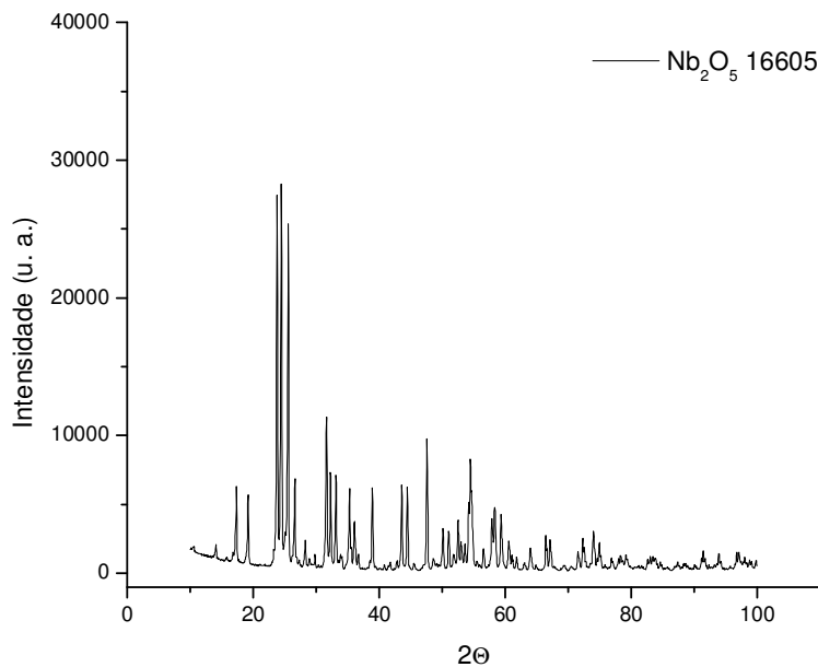
FIG. 4.17 Difratoograma do Nb 2 O 5
