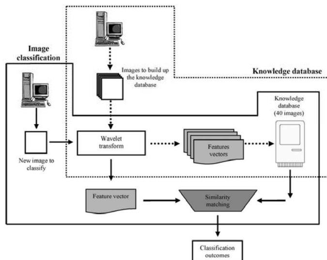
Fig. 2 – Pneumo-CAD prototype scheme showing the construction of the knowledge database in module 1 (dotted line arrows) and further image classification in module 2 (continuous line arrows).
