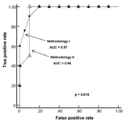
Fig. 6 – ROC curves of methodologies I and II with the Haar wavelet transform. The values of true positive rates (Y axis) versus false positive rates (X axis) vary as a function of the cut-off point for delta.
