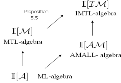
Figure 5.7: \mathbb{I}[\mathcal{IM}] ; an involutive \mathbb{I}[\mathcal{M}] .
