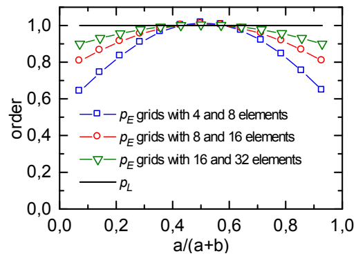
Figure 10. Effective order ( p_E ) for problem B at point 2 for three grid pairs of type shown in Fig. 8a and 8b.
