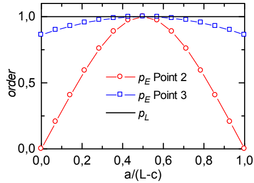
Figure 6. Effective order ( p_E ) for problem A for grids of Fig. 5 with c = 3L/4 .
