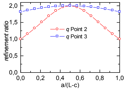
Figure 7. Refinement ratio ( q ) that reproduce asymptotic order ( p_L ) for grids of Fig. 5 with c = 3L/4 .
