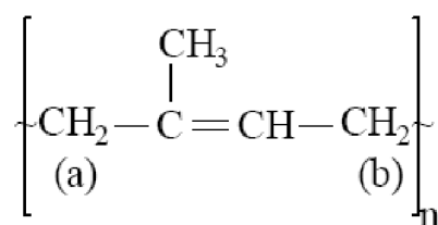
Figura 8 - Cis-1,4-poli-isopreno
