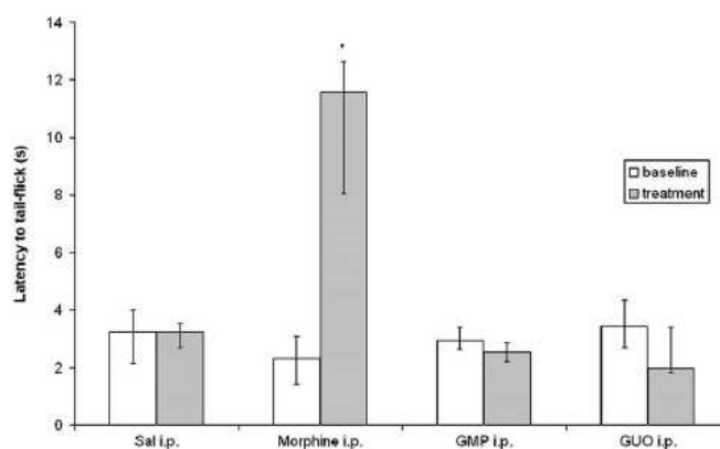
Fig. 4. Effects of GMP, GUO, and morphine on tail-flick measurement. Mice received vehicle (saline 0.9%), morphine, GMP or GUO i.p., 30 min before the tail flick test. For procedure details, see Section 2. Data are medians (interquartile ranges) of the tail-flick latencies on baseline (white columns) and test sessions (grey columns); n = 8 animals per group. Statistical comparison between groups was performed with Kruskal–Wallis test followed by Mann–Whitney test. (*) Indicates a difference from all other groups at P < .05 (Mann–Whitney test).
