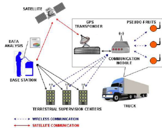
Figure 5. System diagram
