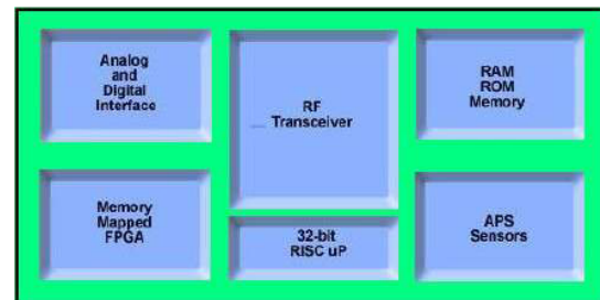
Figure 2. rSoC architecture
