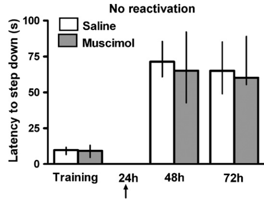
Fig. 3. Muscimol injection 24 h posttraining has no effect in the absence of reactivation. Bars show median and interquartile range values for inhibitory avoidance latencies on the training session and on test sessions performed 48 h and 72 h later. Animals received bilateral intrahippocampal injections of either saline (1 \mu L) (white bars, n=9 ) or muscimol (1.0 \mu g in 1 \mu L of saline) (grey bars, n=7 ) 24 h after the training session with no test session preceding the injections. Subsequent test latencies were not significantly different at either 48 h (Mann–Whitney’s U -test, p = 0.41 ) or 72 h ( p = 1.0 ) post-training.
