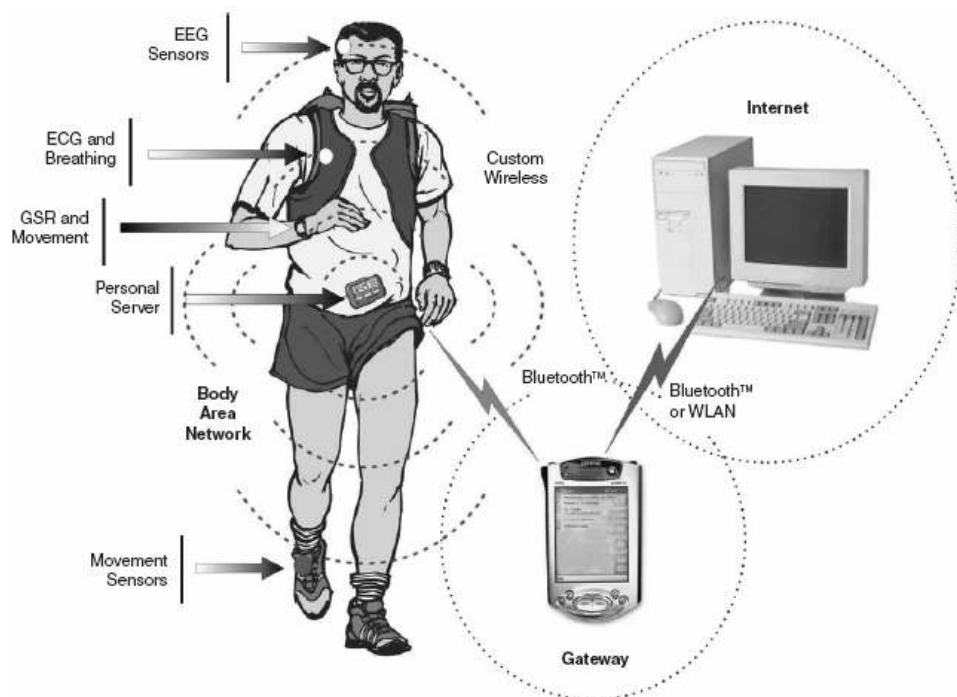
Figura 2.9 - Wireless sensor Body Area Network (WBAN) (JOVANOV, 2006).
