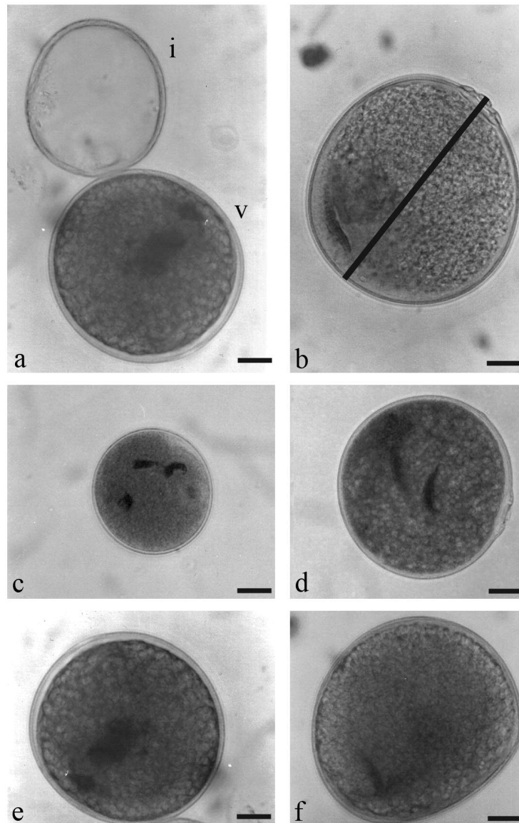
Figure 1: Pollen grains in Triticum species. a) viable (v) and inviable (i) grains; b) measurement of pollen diameter; c) Aegilops tauschii (= T. tauschii ); d) T. durum ; e) T. aestivum ; f) Synthetic form. Bars=10 \mu\text{m} 99x150mm (300 x 300 DPI)
