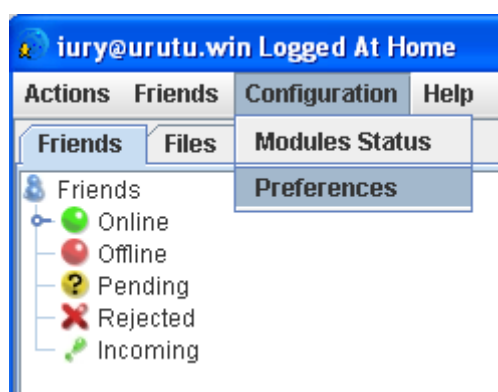
Figura 25 – Menu Preferences
