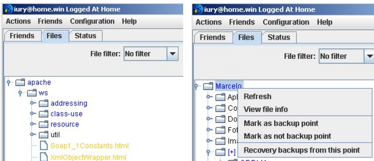
Figura 22 – Aba Files
