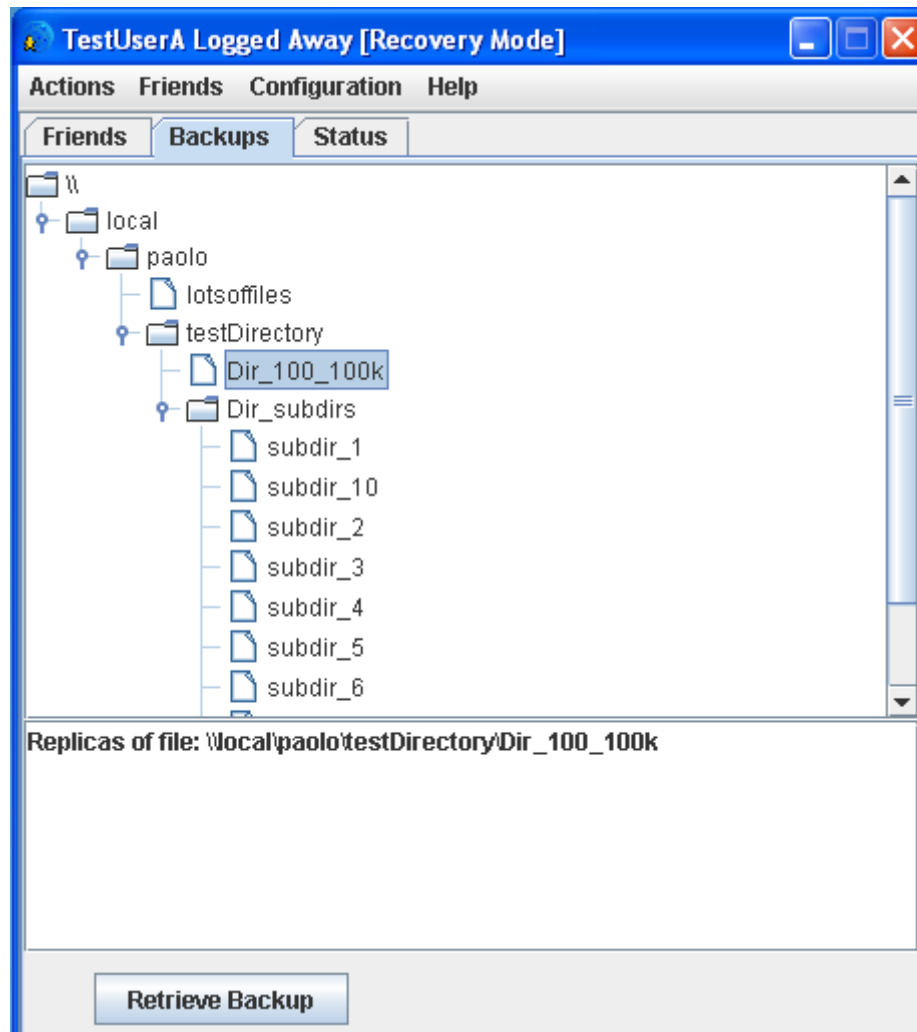
Figura 23 – Aba Backups
