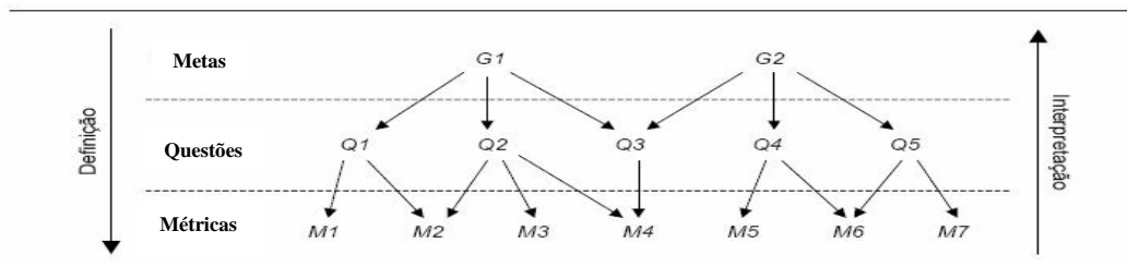
Figura 7 – Método GQM (SOLINGEN; BERGHOUT, 1999)
