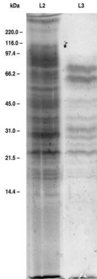
Fig. 1. Protein profile of Dermatobia hominis larvae analyzed by SDS-PAGE. Larvae (L2 and L3) extracts (30 \mu g) were resolved with electrophoresis under denaturing conditions and the gels were silver stained. Molecular mass markers are indicated (kDa). These results are representative of two independent experiments.
