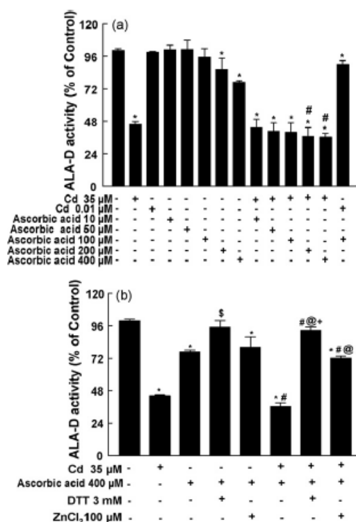
Fig. 4. Effect of ascorbic acid on rat lung \delta -ALA-D inhibition induced by Cd 2+ (a). Effects of DTT and ZnCl 2 on rat lung \delta -ALA-D activity in the presence of ascorbic acid and Cd 2+ (b). Tissue was pre-incubated at 37 °C for 10 min. The enzymatic reaction was initiated by adding the substrate (ALA) in a medium containing 45 mM phosphate buffer, pH 6.8. Data are expressed as mean \pm S.D. \delta -ALA-D activity of control (100%) was of 12.18 \pm 1.66 (mean \pm S.D.) nmol of porphobilinogen/mg protein/h. *: Denoted p < 0.05 as compared to control (one-way ANOVA/Duncan). #: Denoted p < 0.05 as compared to 35 \mu M Cd 2+ (one-way ANOVA/Duncan). +: Denoted p < 0.05 as compared to 35 \mu M Cd 2+ plus ZnCl 2 (one-way ANOVA/Duncan). @: Denoted p < 0.05 as compared to 35 \mu M Cd 2+ plus ascorbic acid (400 \mu M) (one-way ANOVA/Duncan). $: Denoted p < 0.05 as compared to ascorbic acid (400 \mu M) (one-way ANOVA/Duncan). The positive and negative signs mean added or not to the assay.
