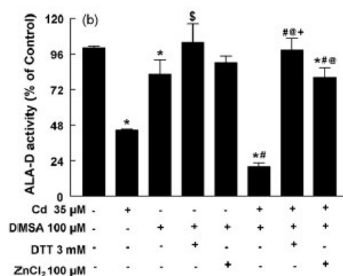
Fig. 3. Effect of DMSA on rat lung \delta -ALA-D inhibition induced by \text{Cd}^{2+} (a). Effects of DTT and \text{ZnCl}_2 on rat lung \delta -ALA-D activity in the presence of DMSA and \text{Cd}^{2+} (b). Tissue was pre-incubated at 37^\circ\text{C} for 10 min. The enzymatic reaction was initiated by adding the substrate (ALA) in a medium containing 45 mM phosphate buffer, pH 6.8. Data are expressed as mean \pm S.D. \delta -ALA-D activity of control (100%) was of 12.18 \pm 1.66 (mean \pm S.D.) nmol of porphobilinogen/mg protein/h. *: Denoted p < 0.05 as compared to control (one-way ANOVA/Duncan). #: Denoted p < 0.05 as compared to 35 \mu\text{M} \text{Cd}^{2+} (one-way ANOVA/Duncan). +: Denoted p < 0.05 as compared to 35 \mu\text{M} \text{Cd}^{2+} plus \text{ZnCl}_2 ( 100 \mu\text{M} ) (one-way ANOVA/Duncan). @: Denoted p < 0.05 as compared to 35 \mu\text{M} \text{Cd}^{2+} plus DMSA ( 100 \mu\text{M} ) (one-way ANOVA/Duncan). $: Denoted p < 0.05 as compared to DMSA ( 100 \mu\text{M} ) (one-way ANOVA/Duncan). The positive and negative signs mean added or not to the assay.
