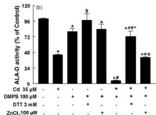
Fig. 2. Effect of DMPS on rat lung \delta -ALA-D inhibition induced by \text{Cd}^{2+} (a). Effects of DTT and \text{ZnCl}_2 on rat lung \delta -ALA-D activity in the presence of DMPS and \text{Cd}^{2+} (b). Tissue was pre-incubated at 37^\circ\text{C} for 10 min. The enzymatic reaction was initiated by adding the substrate (ALA) in a medium containing 45 mM phosphate buffer, pH 6.8. Data are expressed as mean \pm S.D. \delta -ALA-D activity of control (100%) was of 12.18 \pm 1.66 (mean \pm S.D.) nmol of porphobilinogen/mg protein/h. *: Denoted p < 0.05 as compared to control (one-way ANOVA/Duncan). #: Denoted p < 0.05 as compared to 35 \mu\text{M} \text{Cd}^{2+} (one-way ANOVA/Duncan). +: Denoted p < 0.05 as compared to 35 \mu\text{M} \text{Cd}^{2+} plus \text{ZnCl}_2 (one-way ANOVA/Duncan). @: Denoted p < 0.05 as compared to 35 \mu\text{M} \text{Cd}^{2+} plus DMPS (one-way ANOVA/Duncan). $: Denoted p < 0.05 as compared to DMPS (one-way ANOVA/Duncan). The positive and negative signs mean added or not to the assay.
