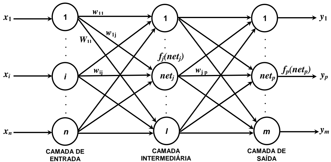
Figura 9 – Rede neural BPN (adaptado de Freeman & Skapura, 1991)
