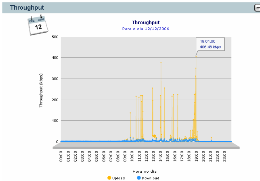
Figura 25 Throughput.
