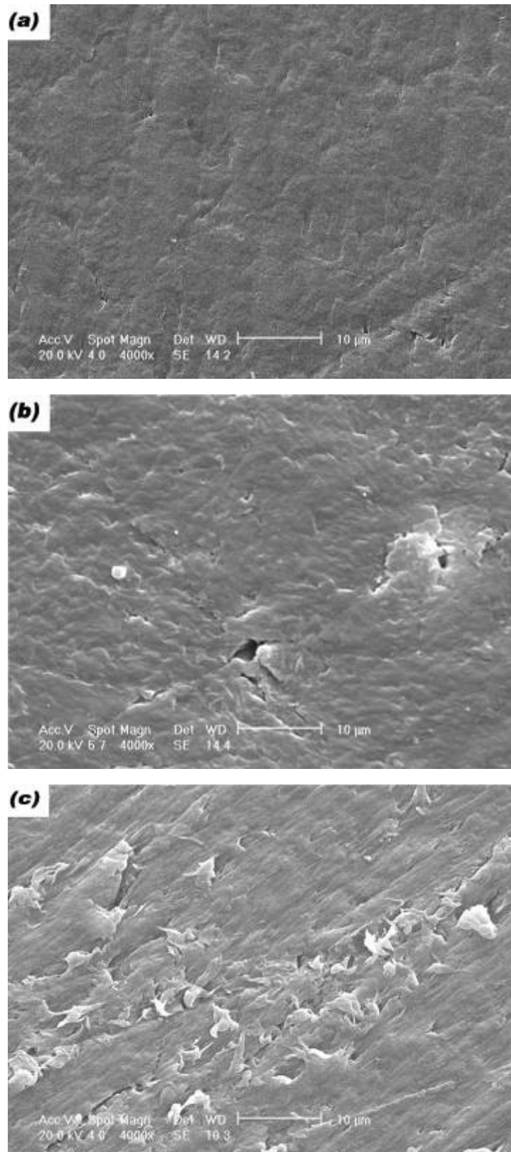
Fig 3.: Scanning electron micrographs at 20 kV and 4000 x magnification of the UHMWPE samples as polished without exposition (a), and irradiated during 6 minutes (b) and 15 minutes (c) with 80 kV x-Ray using a fluoroscopy equipment.
