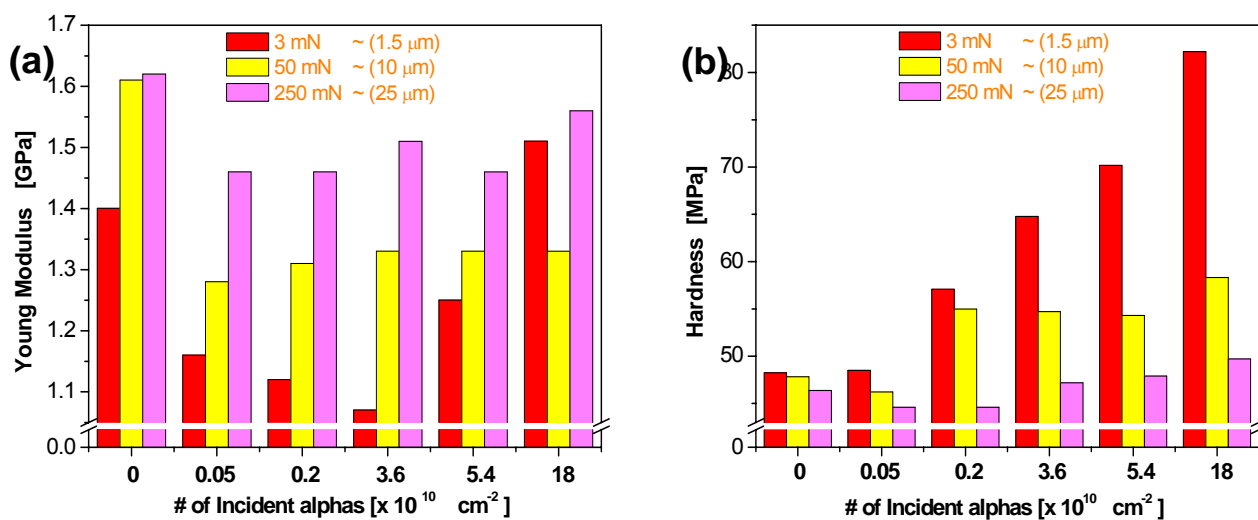
Fig. 2 – (a) Young modulus and (b) Hardness obtained with a nano-indenter using a berkovich tip in the unload cycle for the samples bombarded with alpha particles as function of the dose. The maximum load and depth of testing were 3 mN (~1.5 \mu\text{m} ), 50 mN (~10 \mu\text{m} ), and 250 mN (~25 \mu\text{m} ).
