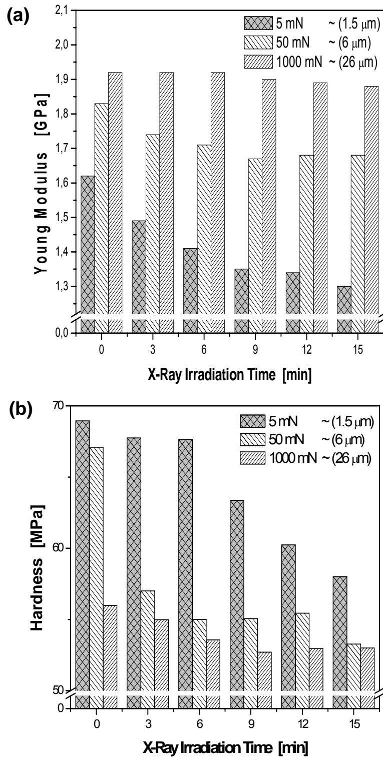
Fig. 2 – (a) Young modulus and (b) hardness obtained with a nanoindenter using a berkovich tip for the UHMWPE samples irradiated with 80 kV x-Ray as function of the exposition time. The maximum load and depth of testing were 5 mN (~ 1.5 μm), 50 mN (~ 6 μm), and 1000 mN (~ 26 μm).
