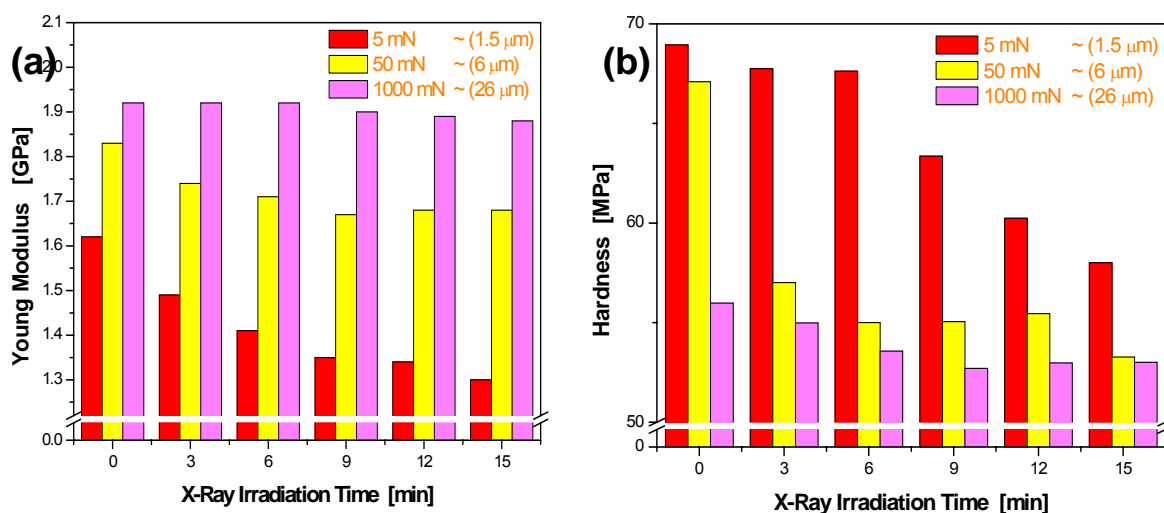
Fig. 4 – (a) Young modulus and (b) hardness obtained with a nanoindenter using a berkovich tip in the unload cycle for the UHMWPE samples irradiated with 70 kV x-Ray as function of the exposition time. The maximum load and depth of testing were 5 mN (~ 1.5 μm), 50 mN (~ 6 μm), and 1000 mN (~ 26 μm).
