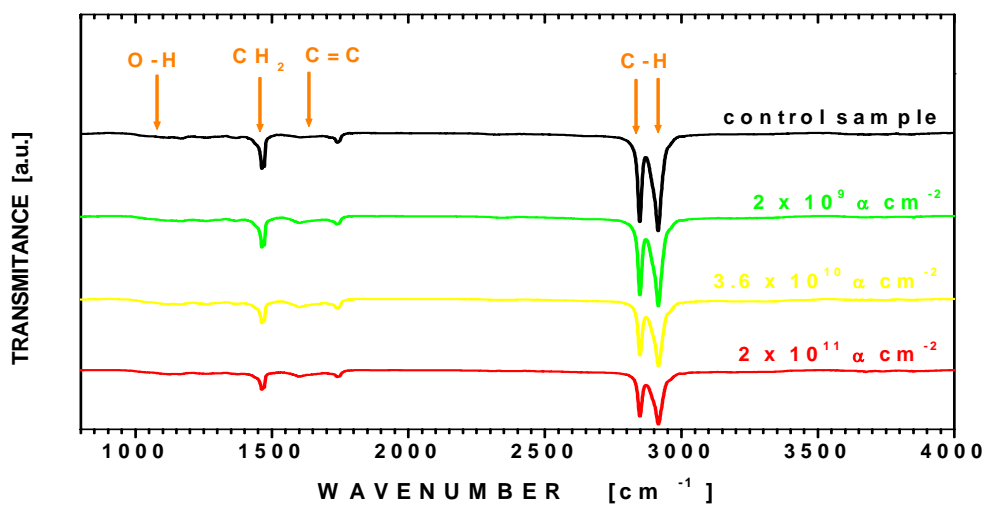
Fig. 1 - ATR - FT-IR spectra of the UHMWPE samples irradiated with 5.4 MeV alpha particles as described in Table 1.
