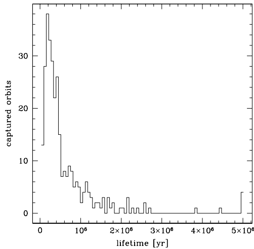
Figure 3. The dynamical lifetimes of the orbits that became captured in any resonance during the simulation, distributed in bins of 60,000 yr. The median lifetime is \tau \sim 3.6 \times 10^5 yr.
