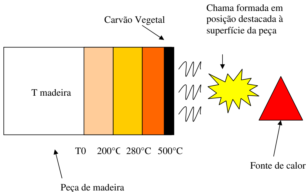
Figura 2.7 – Isoterma 280^{\circ}\text{C} e 500^{\circ}\text{C}
