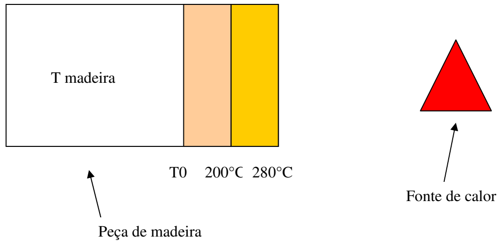
Figura 2.6 – Isoterma 200^{\circ}\text{C} e 280^{\circ}\text{C}
