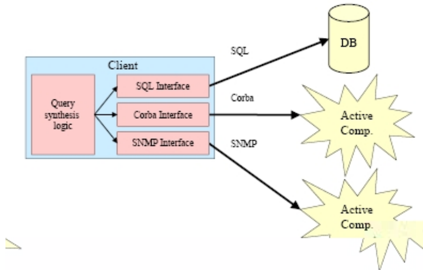
Figura 3.2 – Arquitetura do Service Interface Architecture [1]
