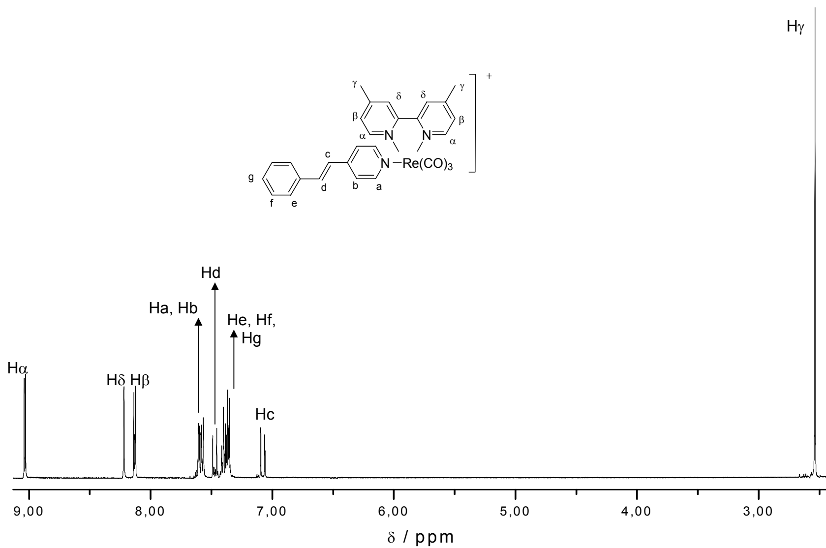
Figura 45. Espectro de ^1\text{H} RMN do composto \text{fac-}[\text{Re}(\text{CO})_3(\text{Me}_2\text{bpy})(\text{trans-stpy})]^+ em \text{CD}_3\text{CN} a 500 MHz. (T = 298 K)
