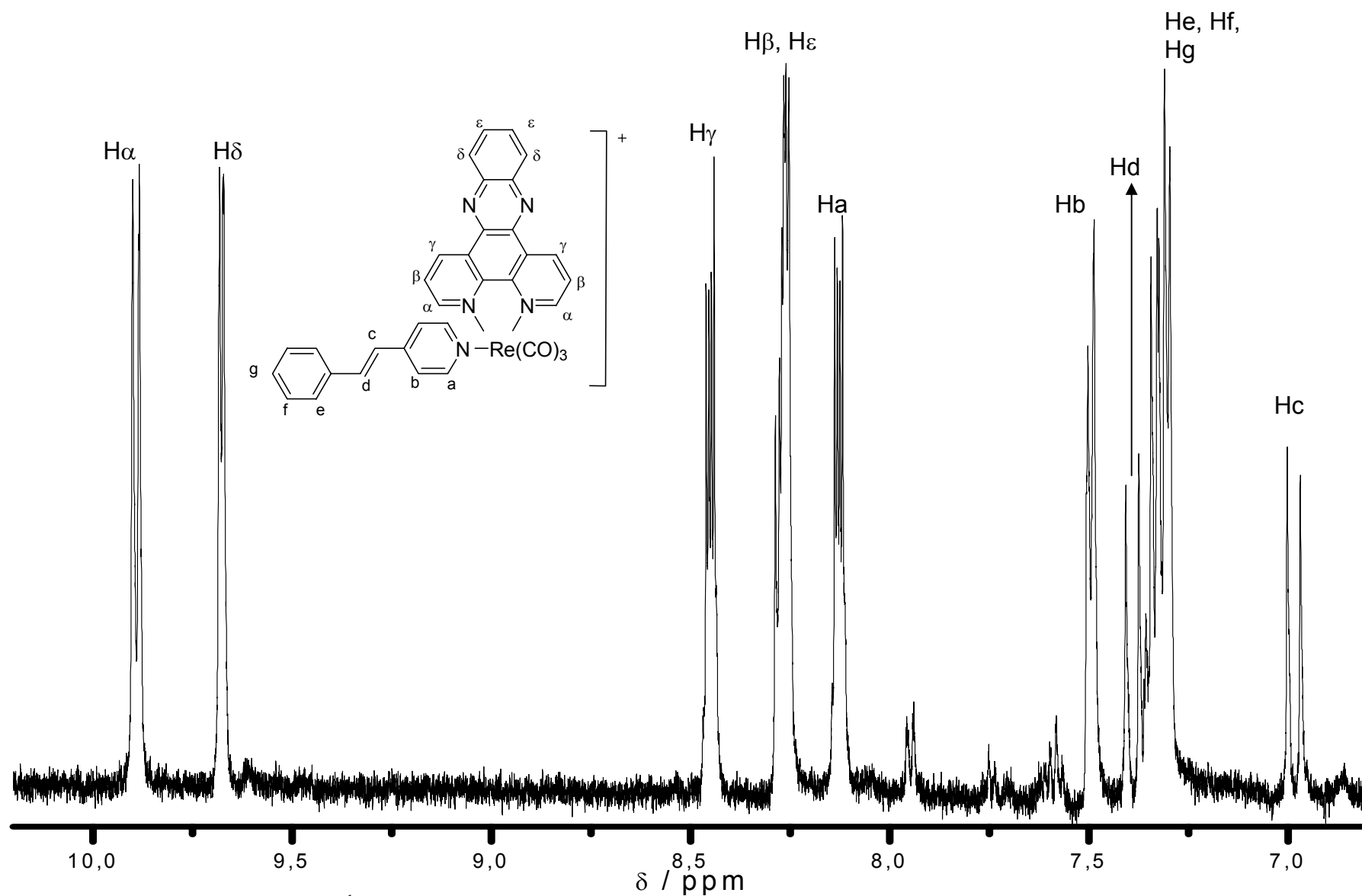
Figura 49. Espectro de ^1\text{H} RMN do composto \text{fac}[\text{Re}(\text{CO})_3(\text{dppz})(\text{trans-stpy})]^+ em \text{CD}_3\text{CN} a 500 MHz. ( T = 298 \text{ K} )
