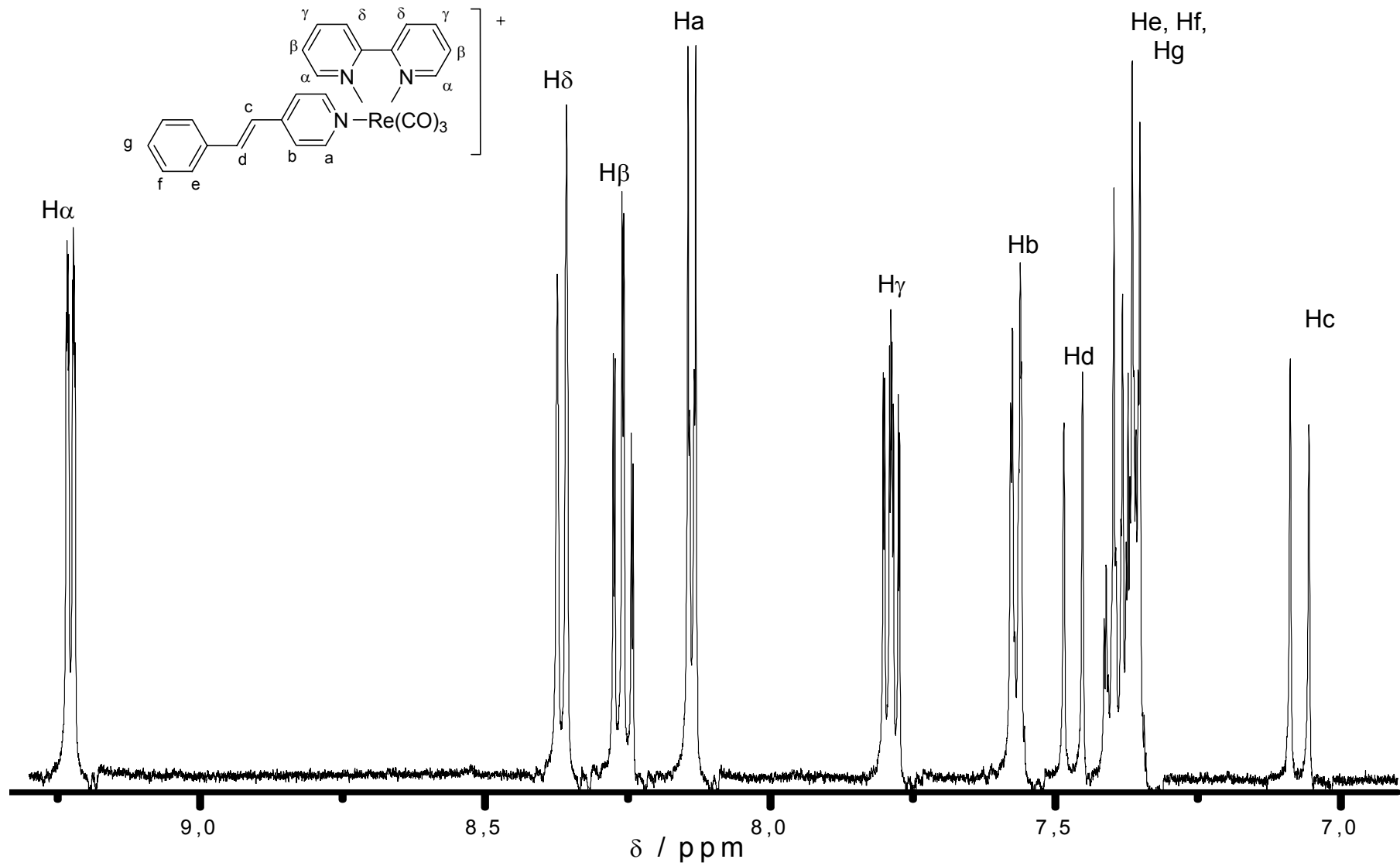
Figura 40. Espectro de ^1\text{H} RMN do composto \text{fac-}[\text{Re}(\text{CO})_3(\text{bpy})(\text{trans-stpy})]^+ em \text{CD}_3\text{CN} a 500 MHz. (T = 298 K)
