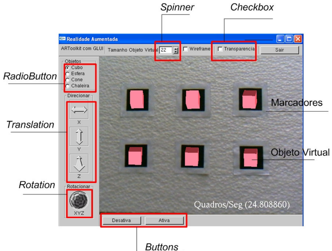
Figura 4.7: Interface de Controle 2D
