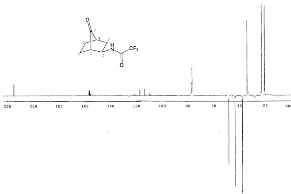
Figura 68. Espectro de RMN de ^{13}\text{C} (APT) da ceto trifluoroacetamida ( \pm )- 80 ( \text{CDCl}_3 , 75 MHz)
