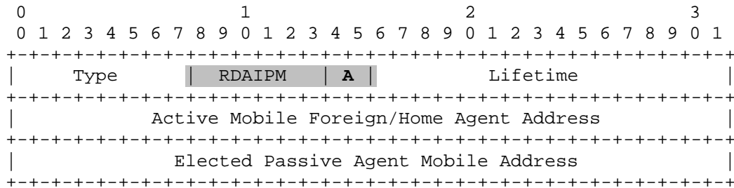
Figura A.8 - Estrutura do MNnodelect Acknowledgement.
