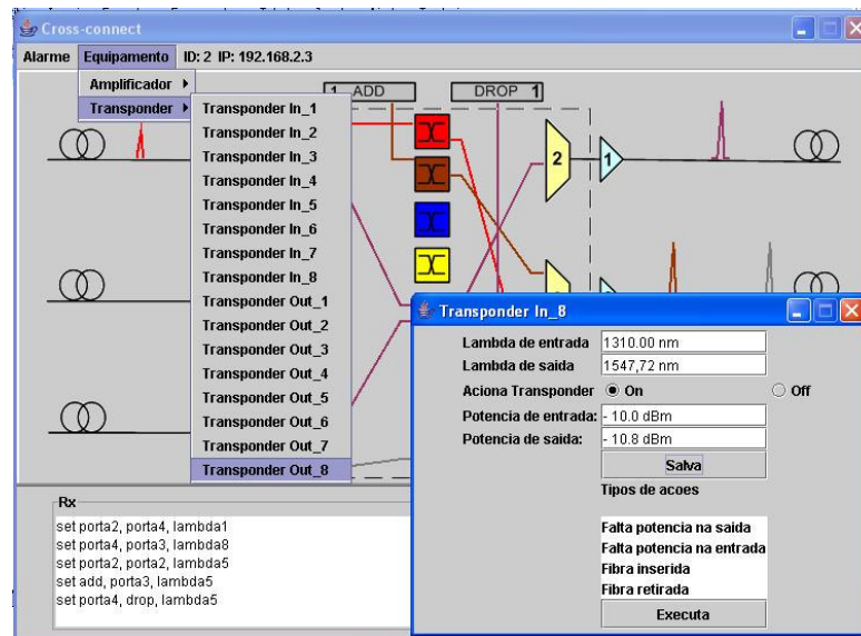
Figura 6.17 – Interface do Transponder
