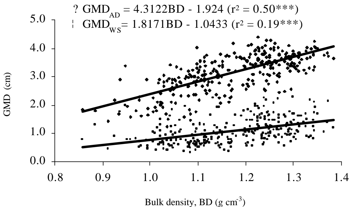
Figure 2.2 - Correlation between bulk density (BD) and geometric mean diameter of air-dry ( GMD_{AD} ) and water stable ( GMD_{WS} ) aggregates for cores sampled at four depths after nine years of applying five soil tillage systems and nutrient sources.
