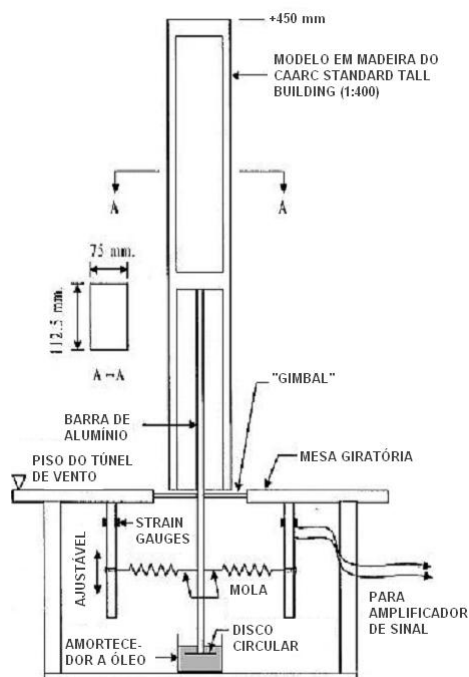
FIGURA 3.2 - CAARC Standard Tall Building modelado com stick
